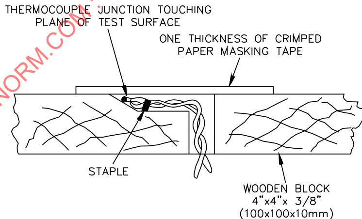
Figure 41.3 Method of mounting thermocouple
