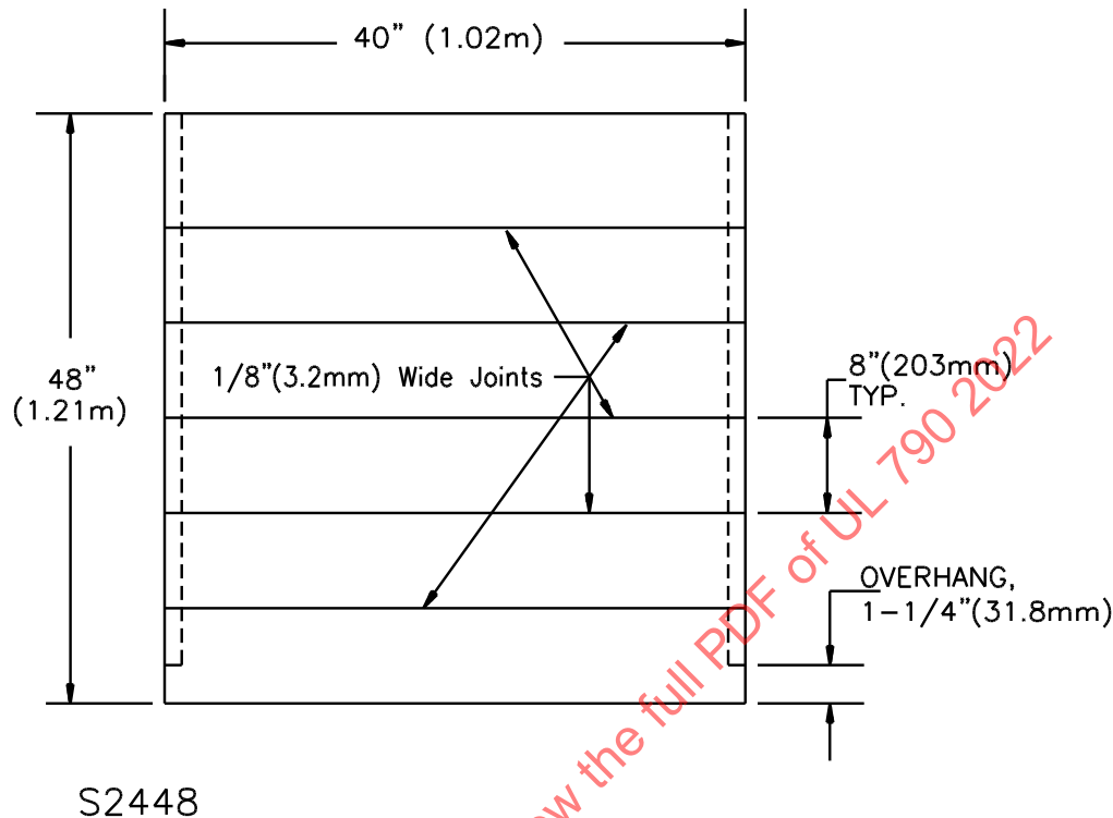
Figure 4.7 Class C Burning-Brand Plywood Deck
