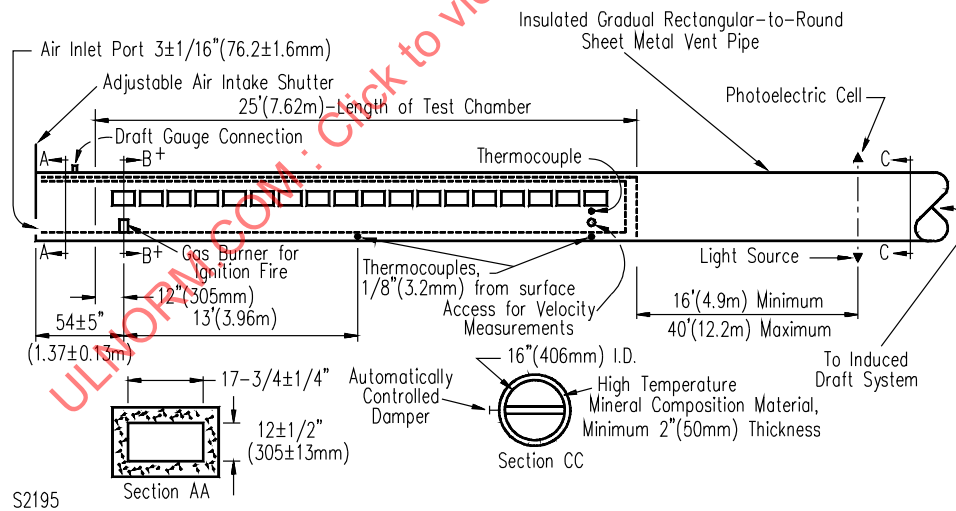
Figure 3.1 Details of test furnace
