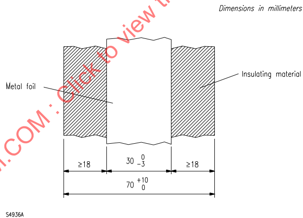
Figure 16 – Final position of mandrel
