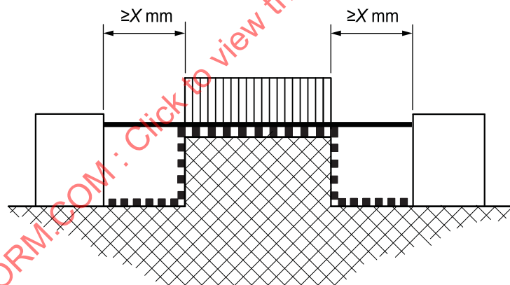
Figure E.5 – Uncemented joint with narrow groove
