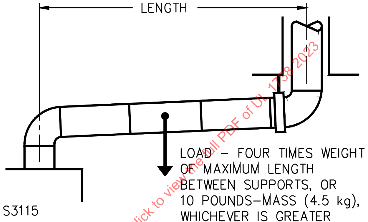
Figure 22.3 Load Test for Vent Elbows
