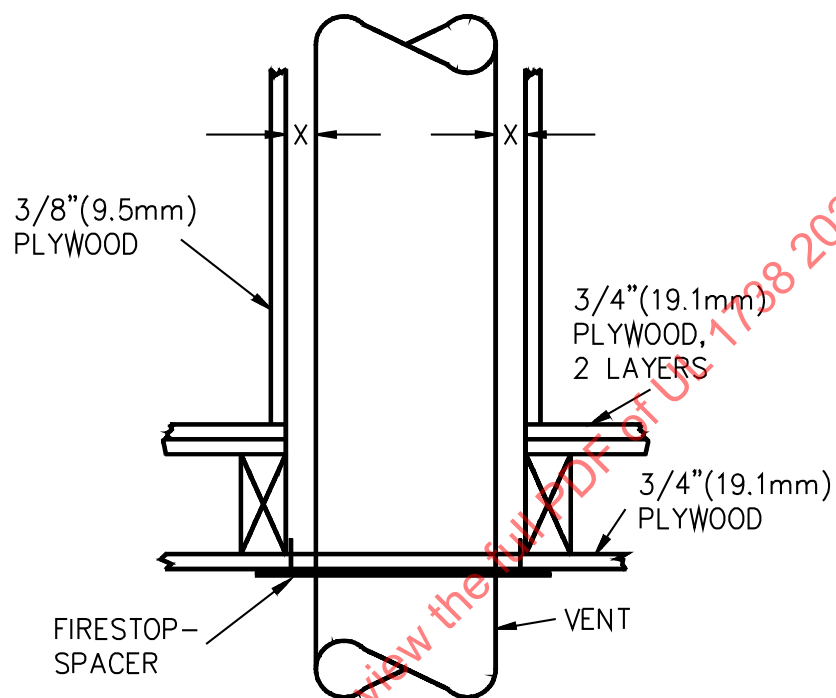
Figure 17.4 Test Structure for Firestop-Spacer Assembly
