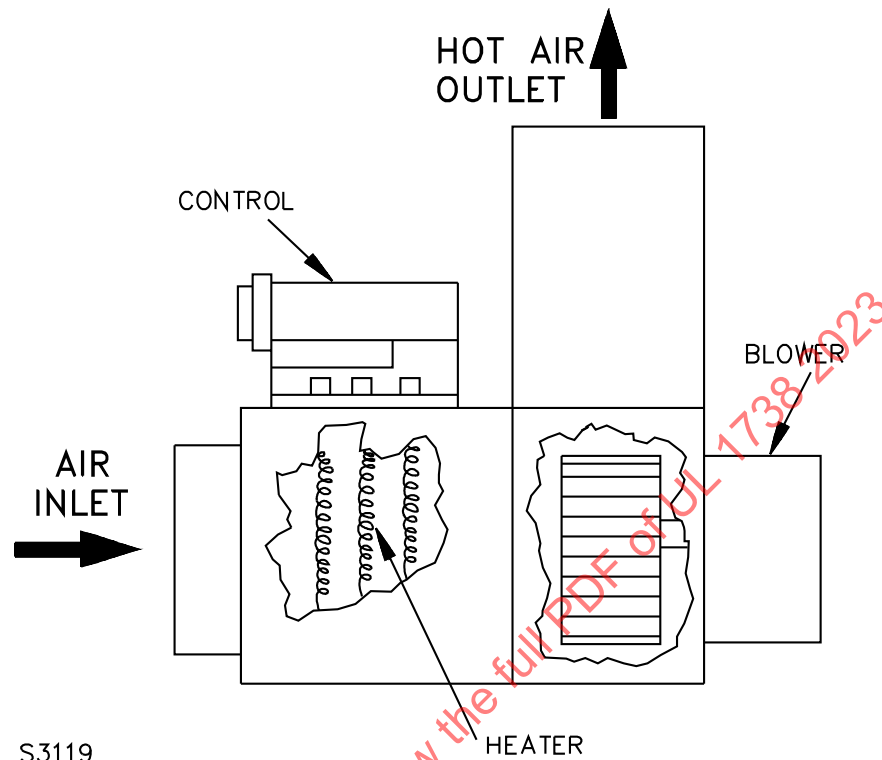
Figure 17.6 Hot Air Blower Heat Producing Assembly
