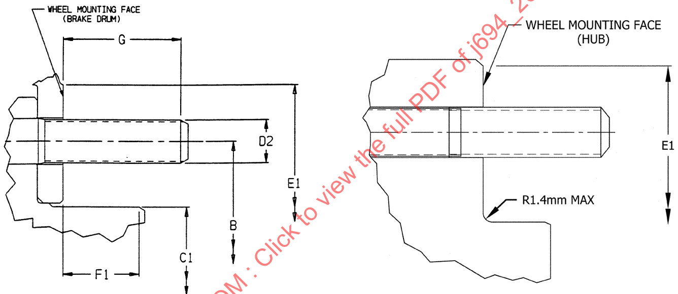
FIGURE 3—HUB OR DRUM INTERFACE DIMENSIONS
