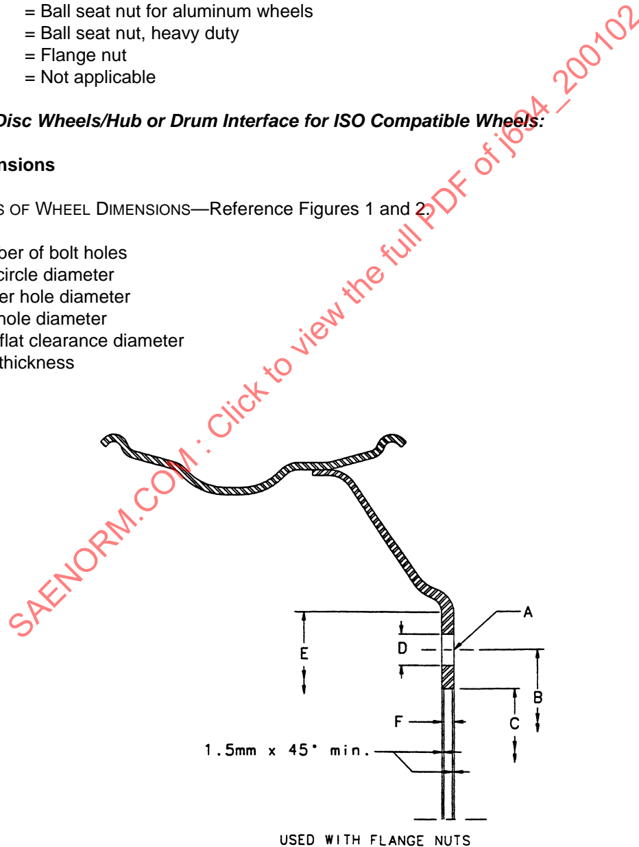
FIGURE 1—FERROUS DISC WHEEL
