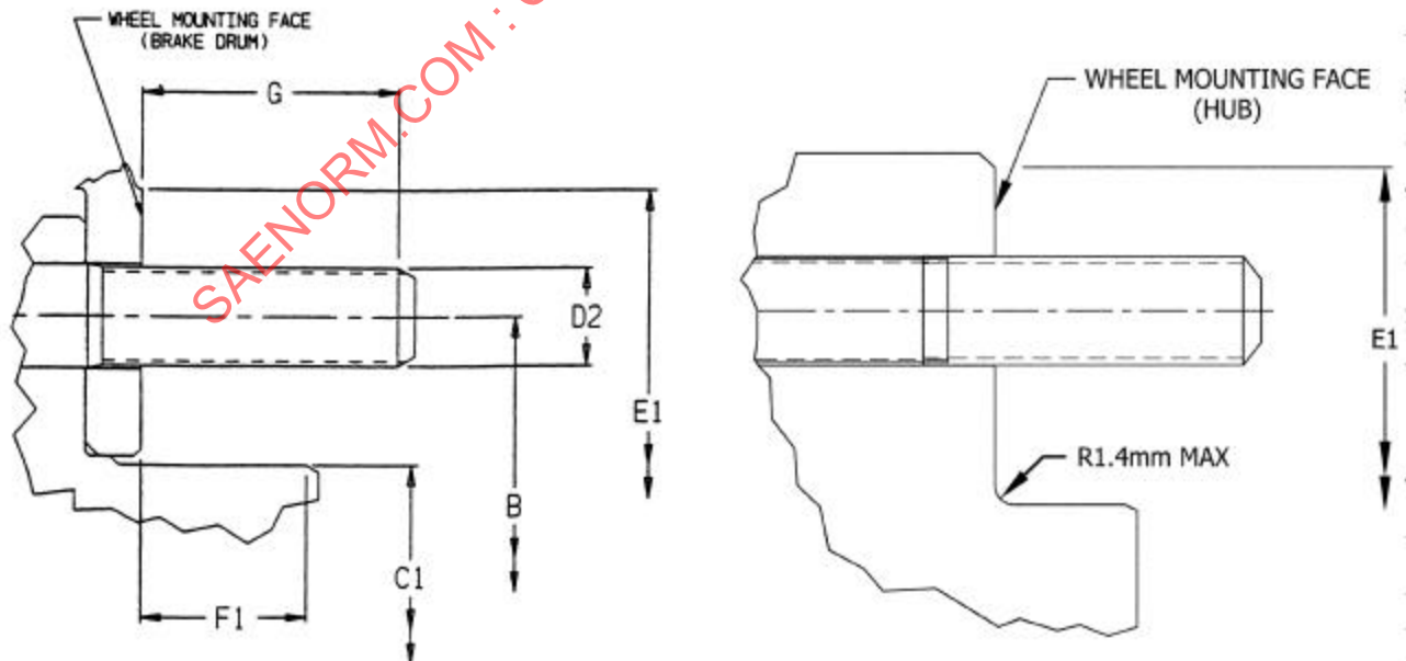
FIGURE 7—HUB OR DRUM INTERFACE DIMENSIONS
