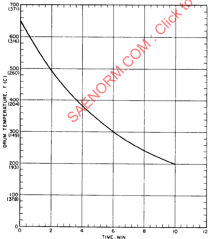
FIG. 4—STANDARD DRUM COOLING CURVE, FRICTION MATERIALS TEST MACHINE
