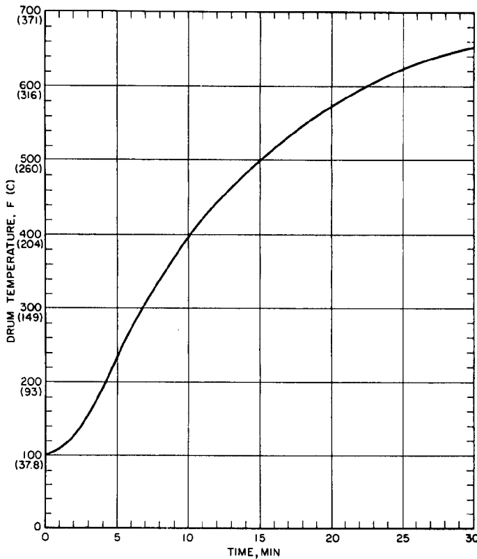
FIG. 3—STANDARD DRUM HEATING CURVE, FRICTION MATERIALS TEST MACHINE
