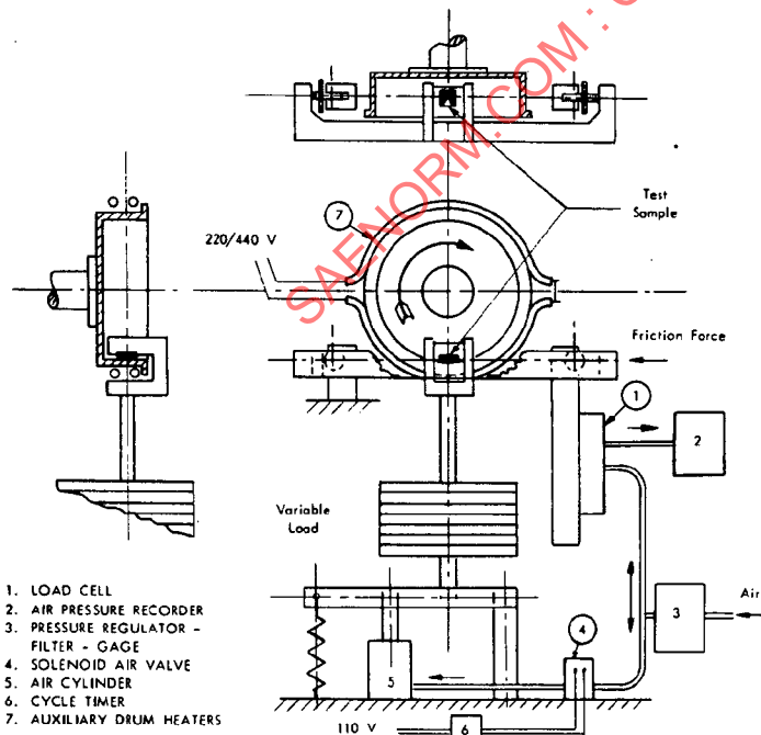
FIG. 1—SCHEMATIC DIAGRAM OF FRICTION MATERIALS TEST MACHINE
