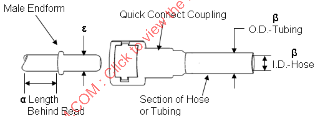
FIGURE 1 - CONNECTOR NOMENCLATURE
