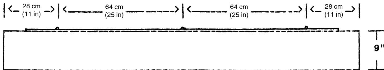
FRONT VIEW
