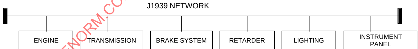
FIGURE 1—SINGLE NETWORK (SPECIFIC ATTACHED DEVICES ARE ONLY AS EXAMPLES)
