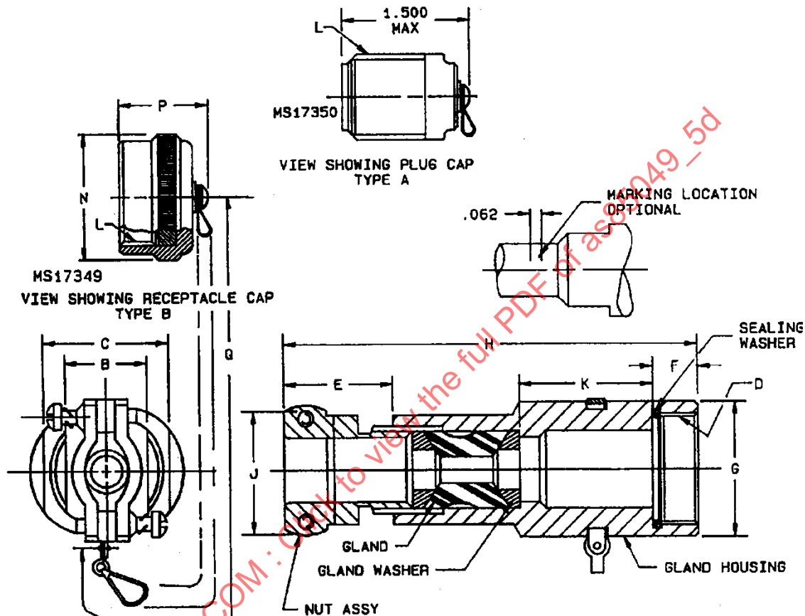
CONFIGURATION 1A - STYLE 1 CABLE SEALING
