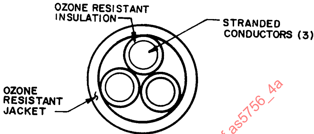
FIGURE 1 – EXAMPLE OF 3 CONDUCTOR CABLE
