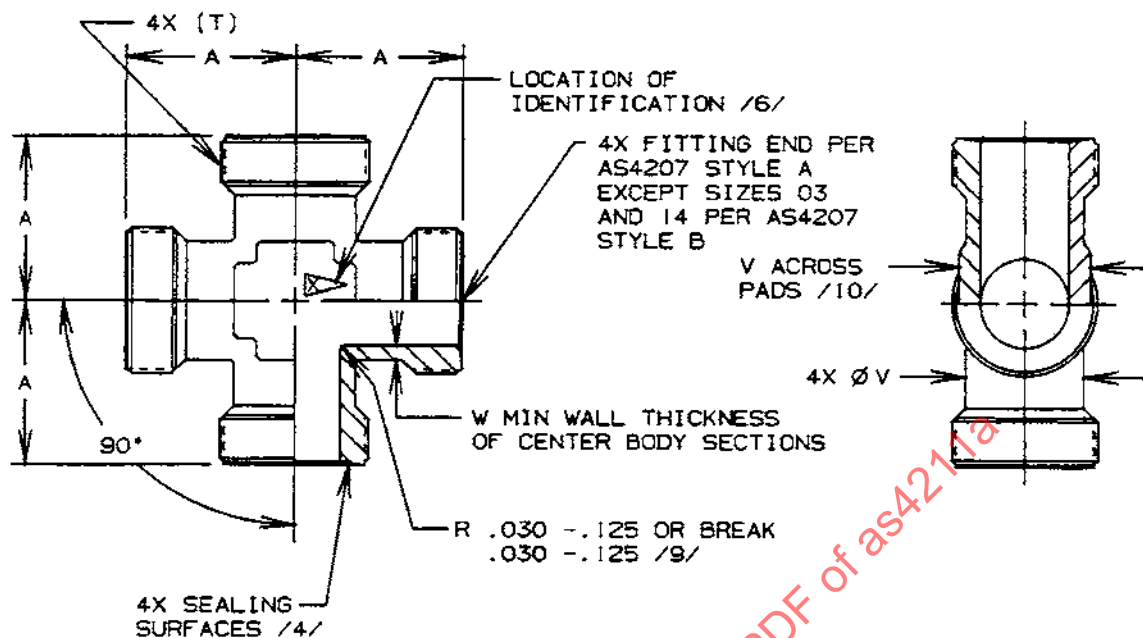
FIGURE 1 - FITTING, CROSS
