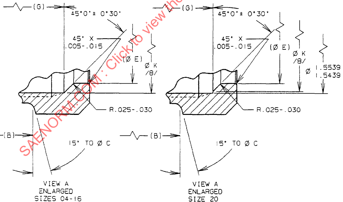
FIGURE 1 - NUT, LIGHTWEIGHT, FLARELESS
