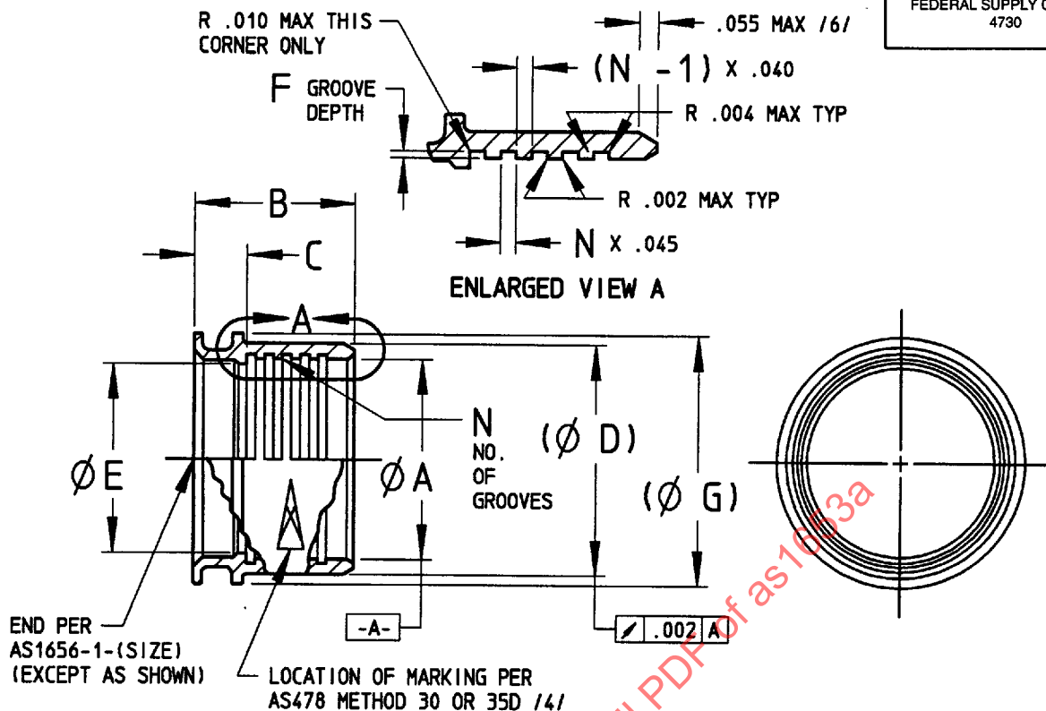
FIGURE 1 - FERRULE
