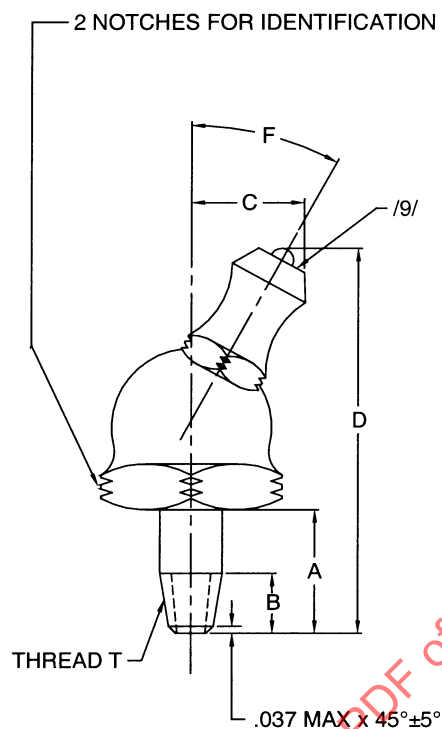
FIGURE 2 - FITTING, ELBOW
