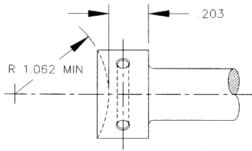
OPTIONAL METHOD OF SLOTTING
