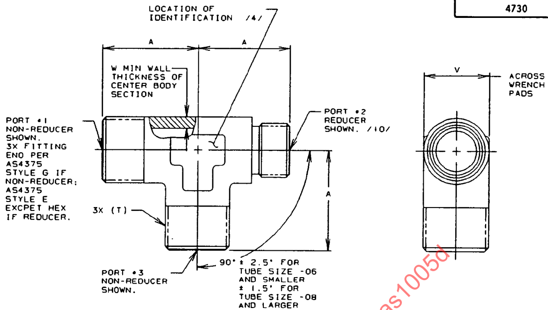
FIGURE 1 - TEE, FLARELESS
