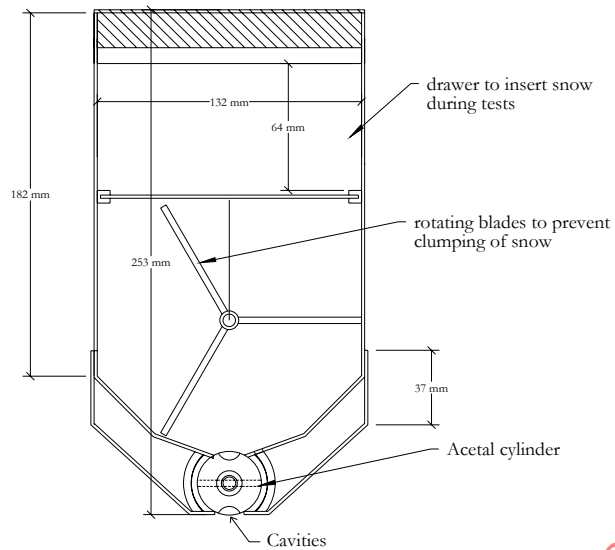
FIGURE 8 - CROSS-SECTION OF SNOW BOX
