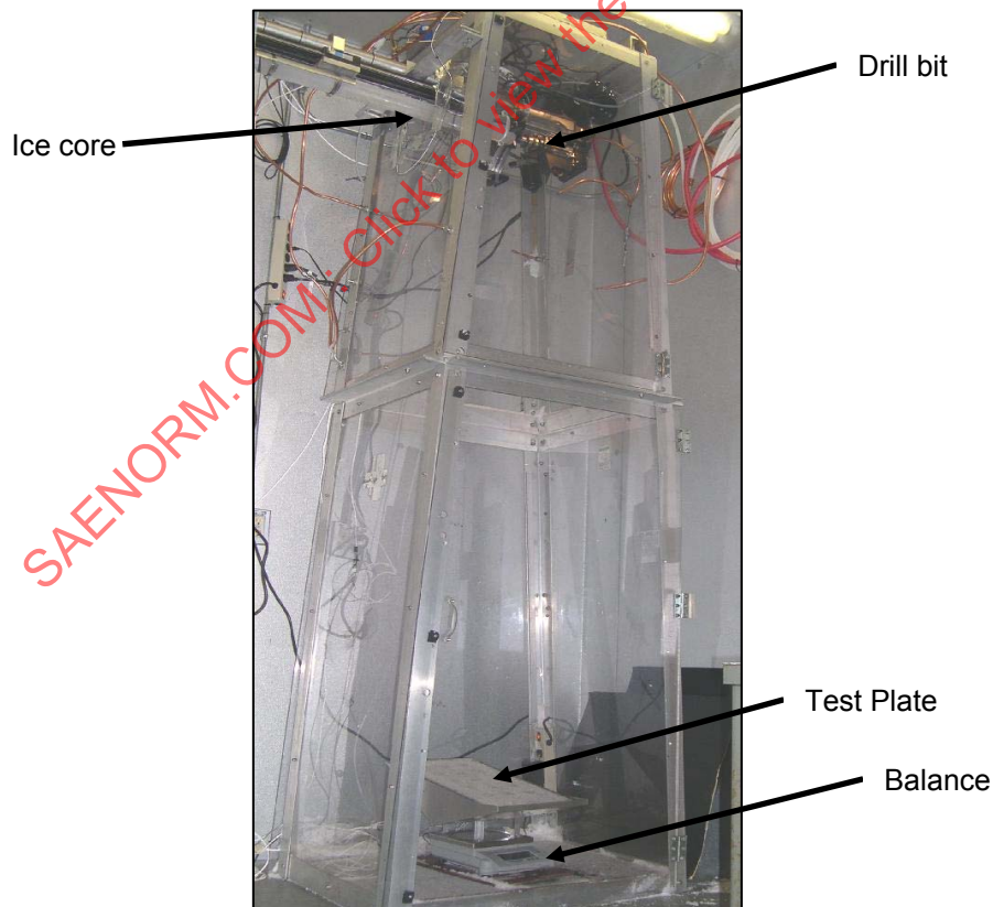
FIGURE 10 - EXAMPLE OF A SIMULTANEOUS ARTIFICIAL SNOW MACHINE AND FLUID TESTING SYSTEM
