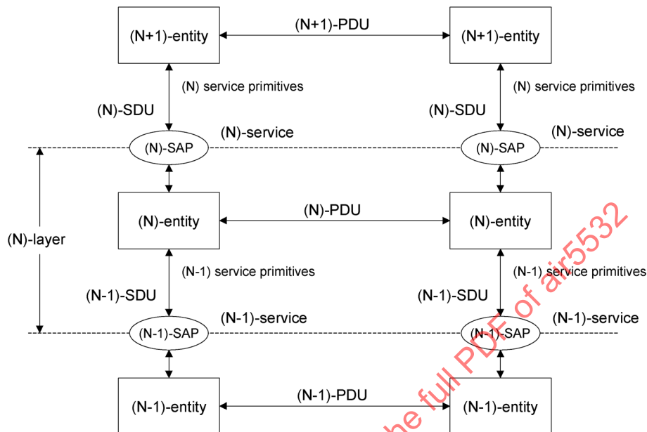
FIGURE 3 - Generic Model of Single (N)-Protocol Layer
