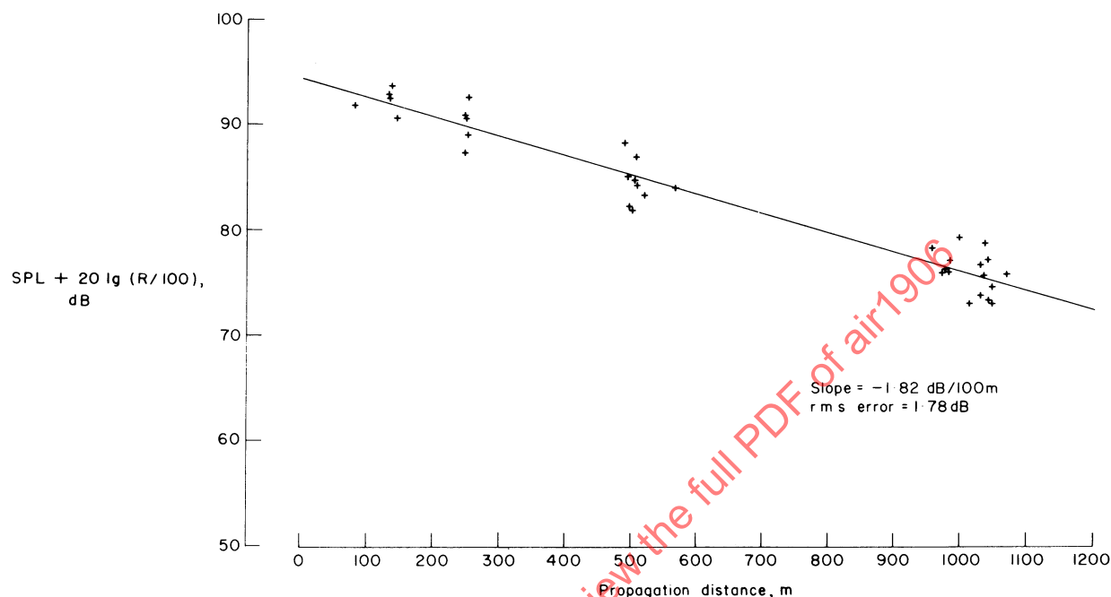
Sketch A.3.7 Regression analysis for the one-third-octave-band sound pressure level at 2.0 kHz, under the flight path.
