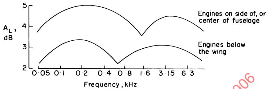
Sketch A.3.5 Typical variations of lateral attenuation with frequency.
