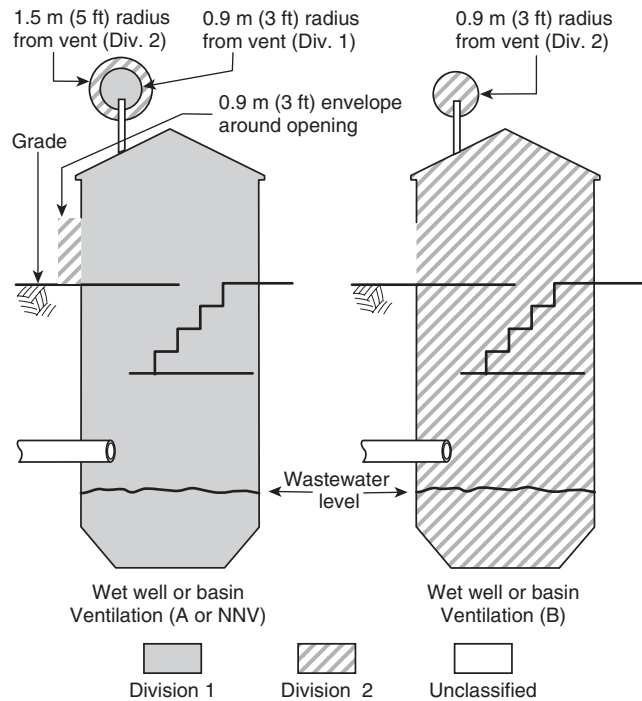
FIGURE A.4.2(c) Wet Well or Basin Serving Separate or Combined Sanitary Sewer; Illustration of Table 4.2, Rows 16 and 34.
