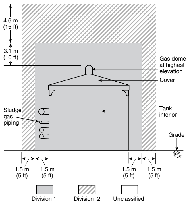
FIGURE A.6.2(a) Anaerobic Digester with Fixed or Floating Cover Abovegrade not Enclosed in a Building; Illustration of Table 6.2(a), Rows 15a and 15b.
