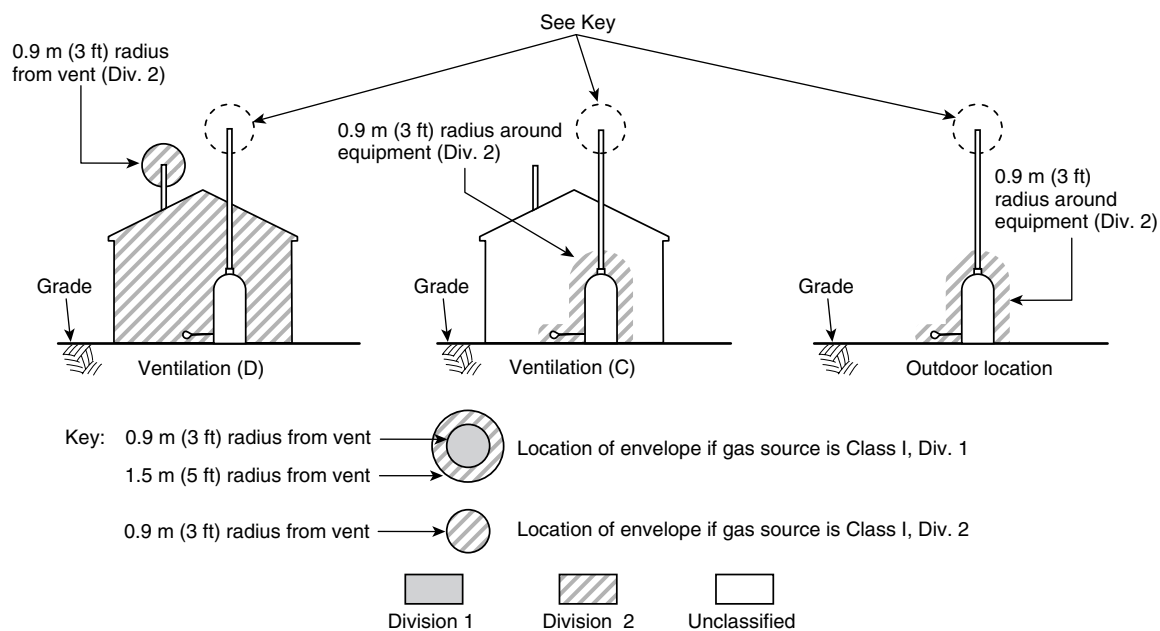
FIGURE A.4.2(g) Odor-Control System Location Physically Separated from Wet Well; Illustration of Table 4.2, Row 20.
