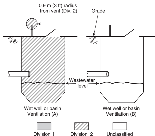
FIGURE A.4.2(b) Wet Well or Basin Serving a Residential Sewer; Illustration of Table 4.2, Row 11.
