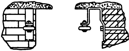
Figure B-13 Stay roll.
