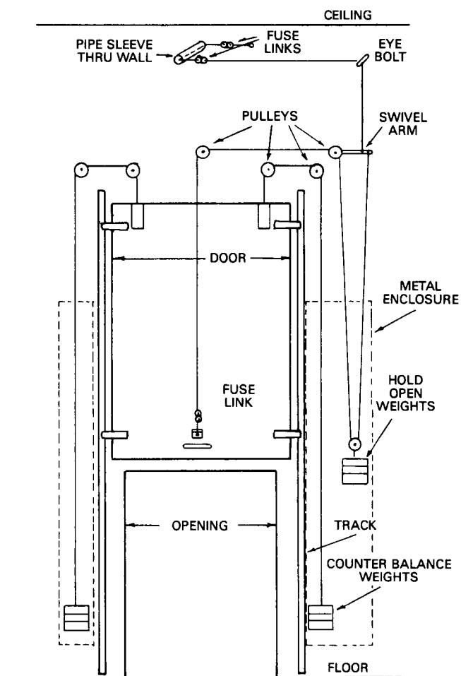
Figure B-46 Closing devices for vertically sliding door.
