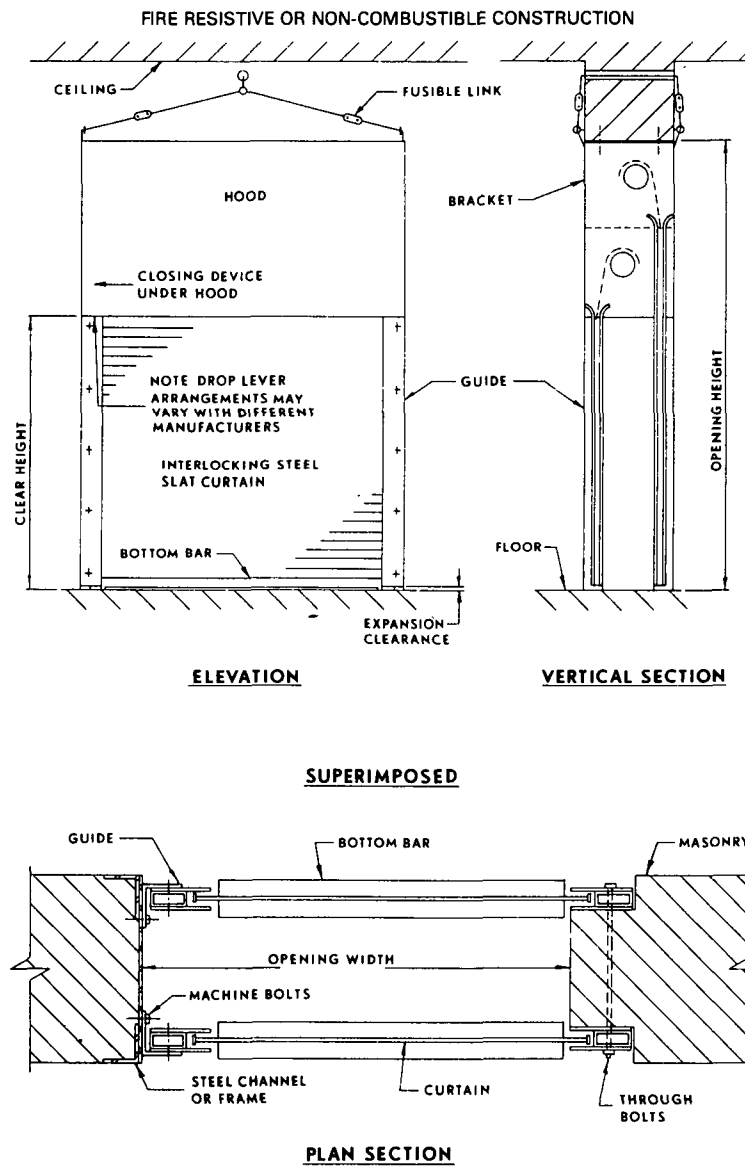
Figure B-50 Rolling steel doors between jamb superimposed mounted.
