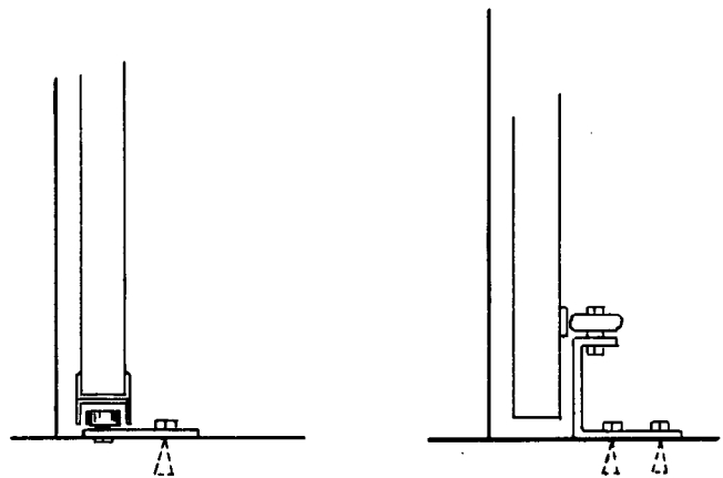
Figure B-15A Stay rolls.
