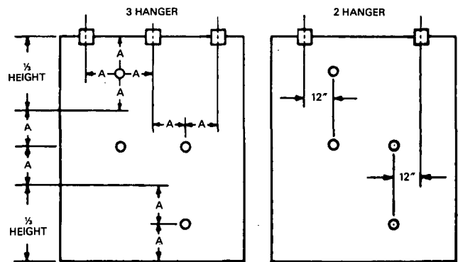
FOUR-3 IN. DIA. VENT HOLES REQUIRED FOR DOORS OVER 9 FT.-0 IN. AND UP TO AND INCLUDING 12 FT.-4 IN. IN HEIGHT
