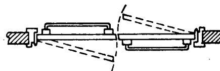
Figure B-25 Double egress door and frame.
