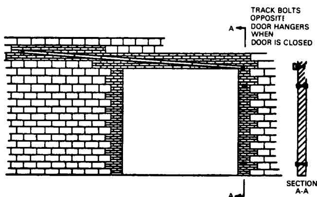
Figure B-18 Hollow concrete masonry wall prepared for single tinclad or sheet metal sliding door, standard method.
