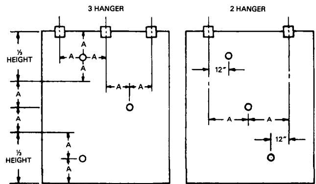
THREE-3 IN. DIA. VENT HOLES REQUIRED FOR DOORS UP TO AND INCLUDING 9 FT.-0 IN. IN HEIGHT A = EQUAL DISTANCES FROM CENTERLINES
