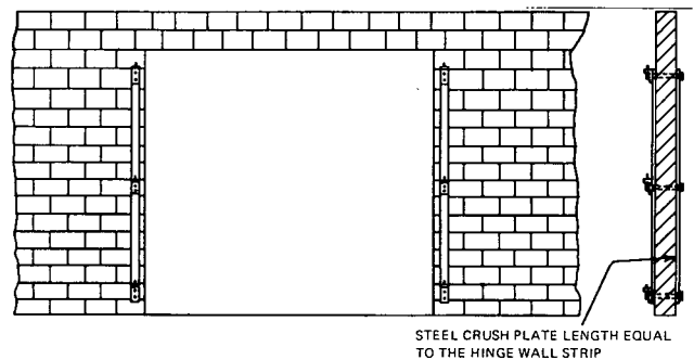
Figure B-17 Hollow concrete masonry wall prepared for doors swinging in pairs - lap mounted.
