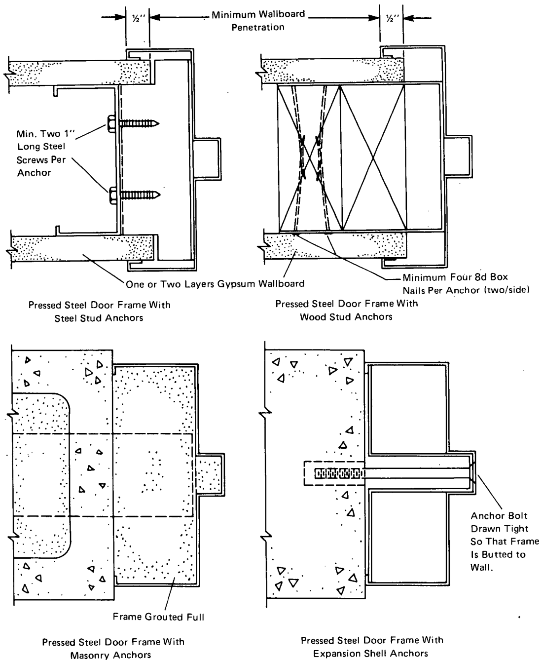
Figure B26-A Typical pressed steel door frame installation.
