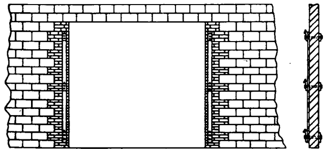
Figure B-16 Hollow concrete masonry wall prepared for doors swinging in pairs - lap mounted, standard method.
