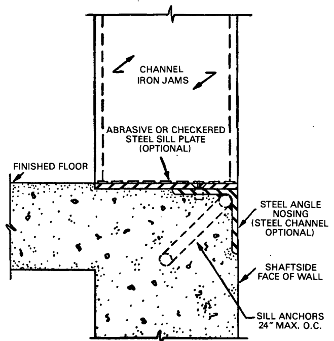
Figure B-58 Sill section showing recommended construction for biparting doors.
