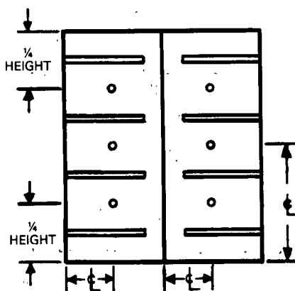
Figure B-33 Location of vent holes for swinging doors.
