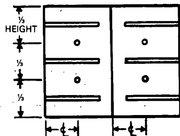
Figure B-32 Closing devices for doors swinging in pairs.
