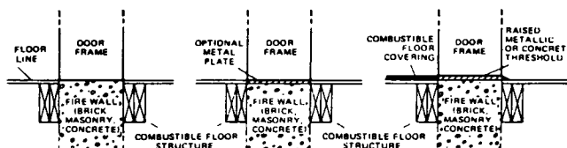
Figure B-2 Noncombustible sill used with combustible floors for doors swinging into steel frame.
