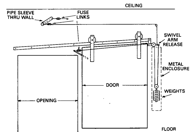
Figure B-35 Closing devices for single sliding door (inclined track).
