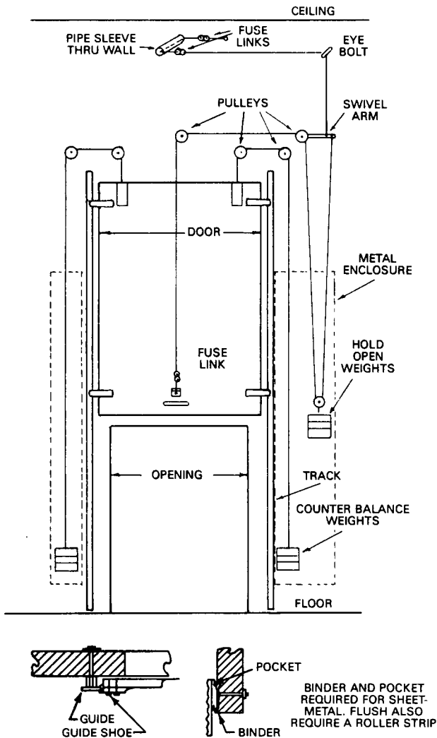
Figure B-45 Vertically sliding door.
