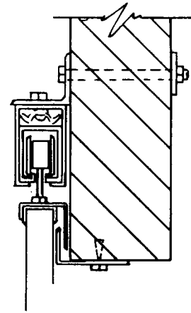
Figure B-44B Binder Arrangements.
