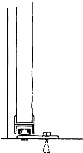
Figure B-15A Stay rolls.
