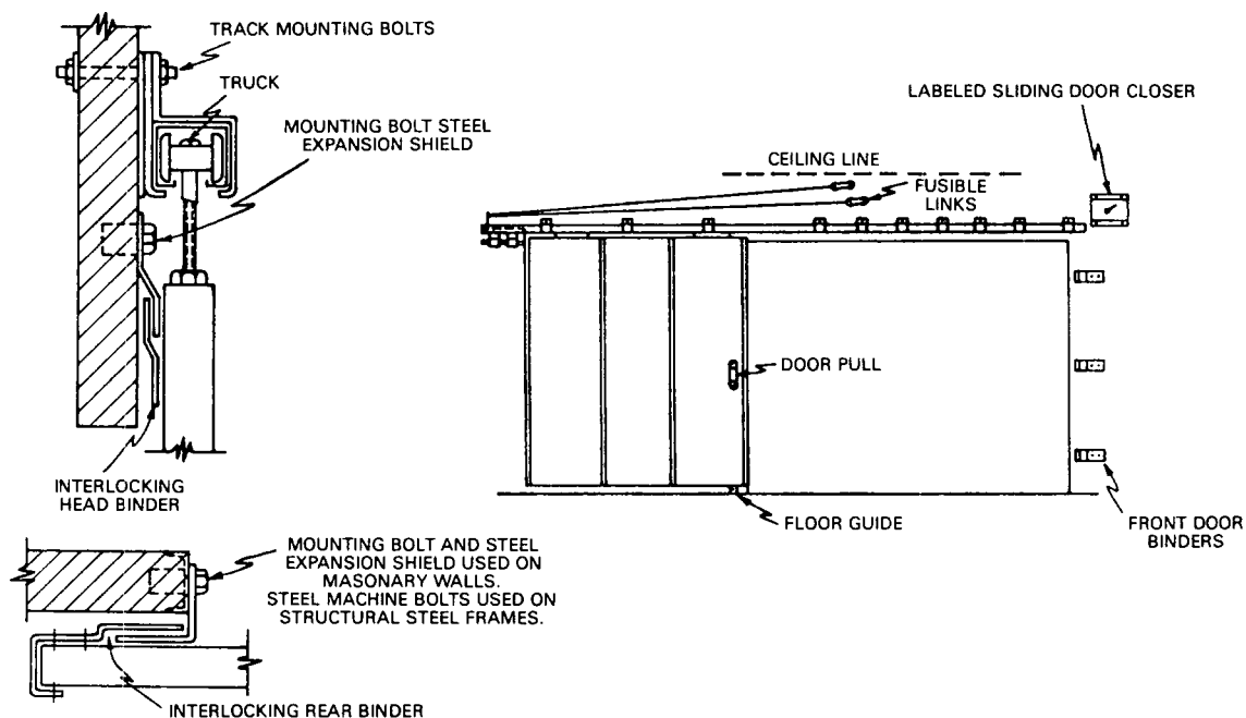
Figure B-43 Horizontally sliding hollow metal door.
