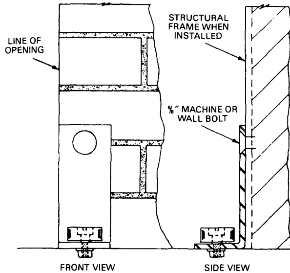
Figure B-15 Concealed type stay roll.
