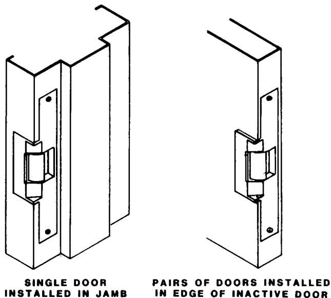
Figure B-65 Typical "Electric Strike" for single swing and for pairs of doors when permitted by individual listings.
