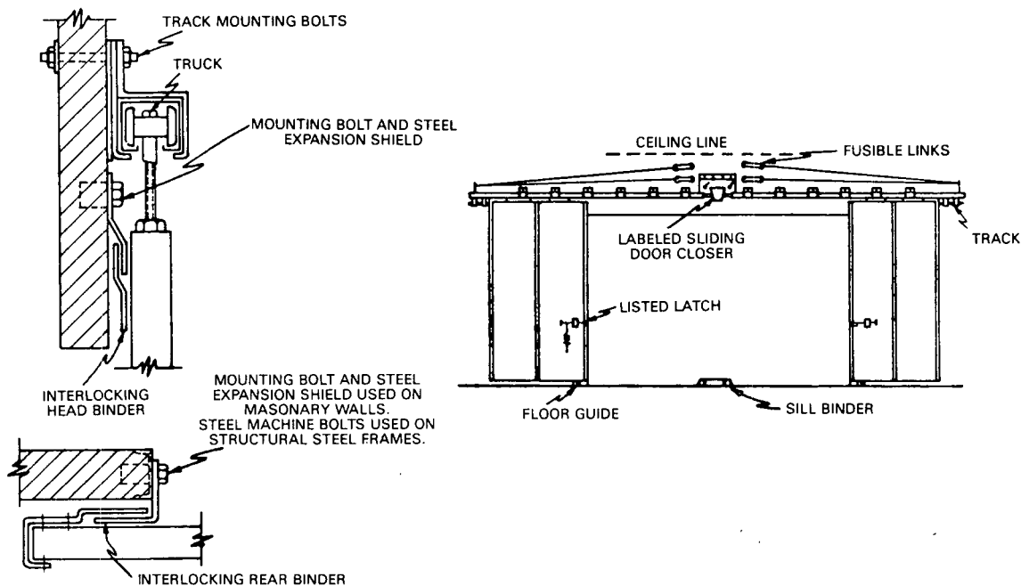
Figure B-44 Center parting horizontally sliding hollow metal door.
