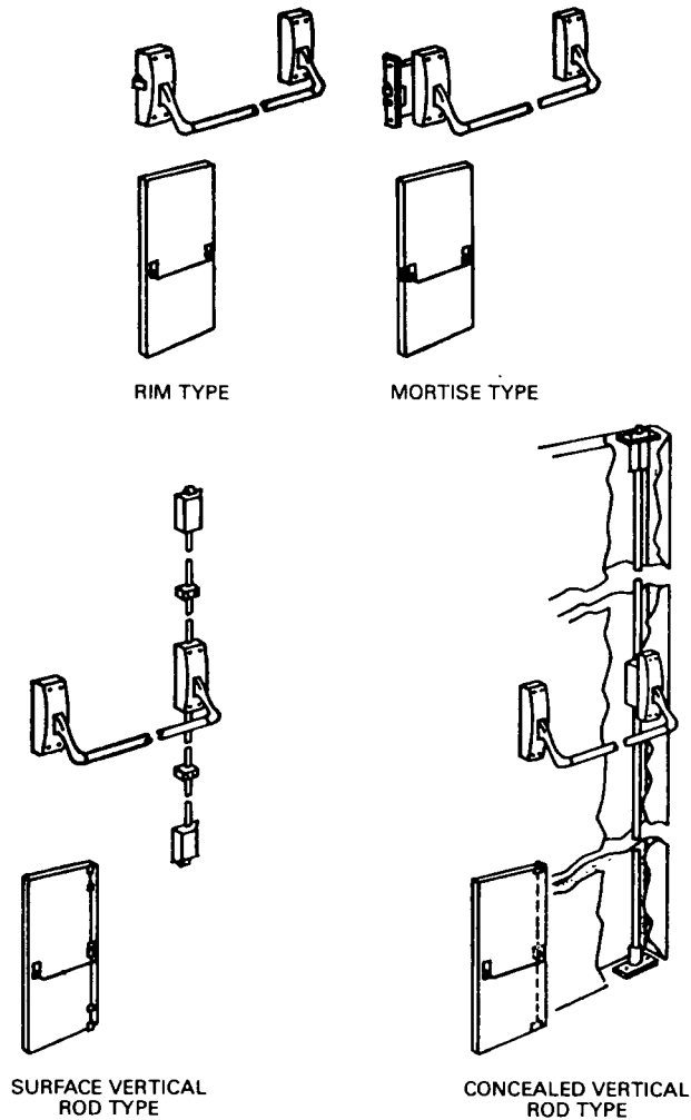
Figure B-24 Types of fire exit hardware.
