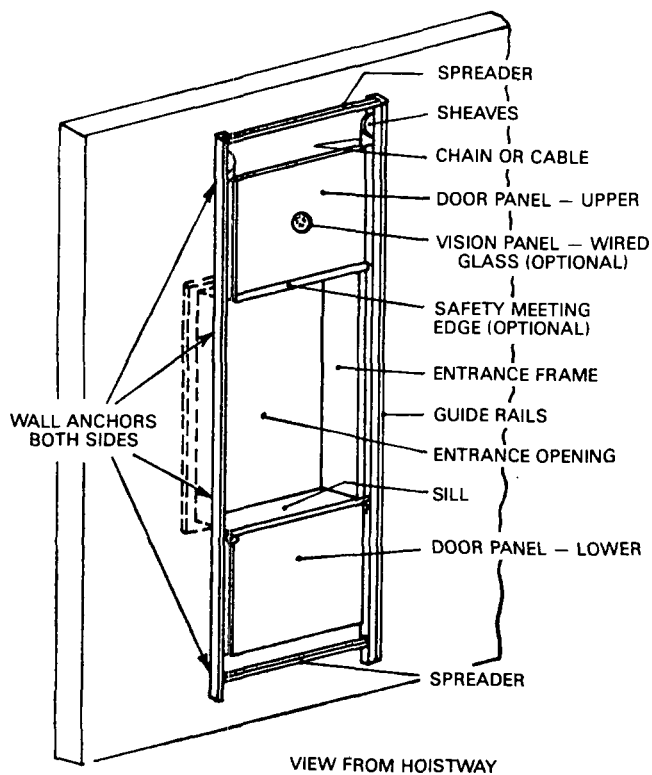
Figure B-57 Dumbwaiter assembly installation for vertically biparting doors.
