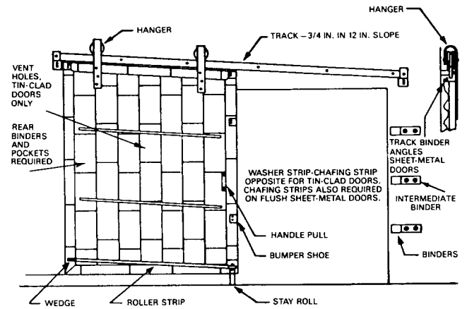
Figure B-34 Single sliding door (inclined track).
