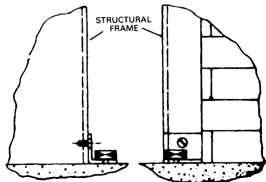
Figure B-14 Concealed type stay roll.
