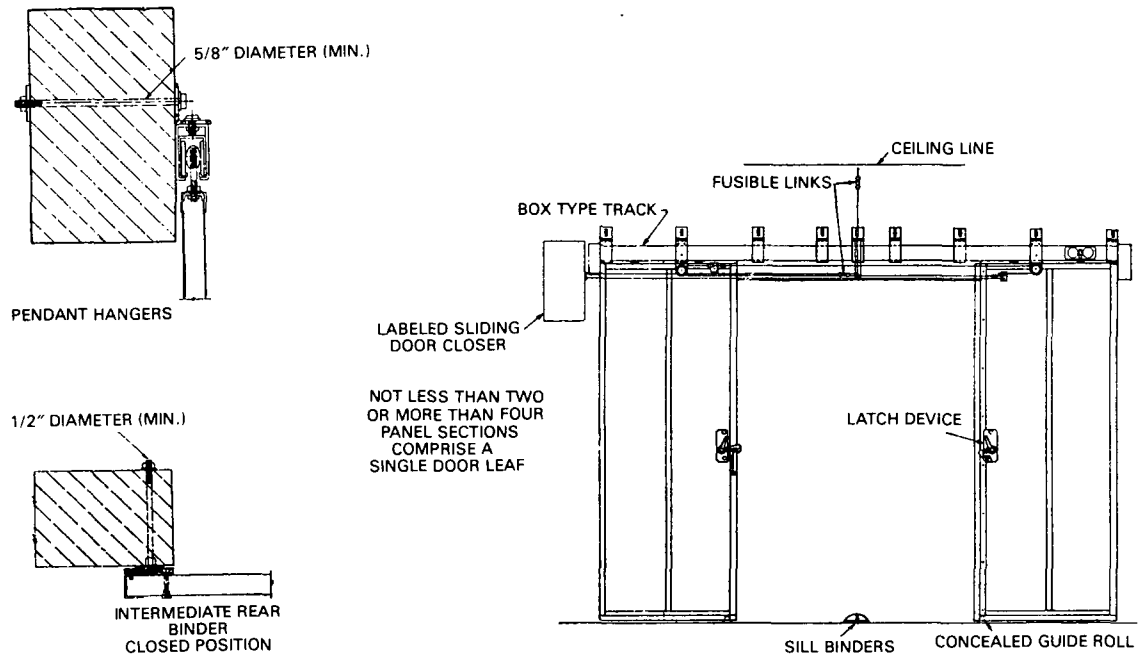
Figure B-42 Center parting horizontally sliding composite door.
