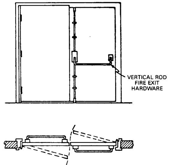
Figure B-25 Double egress door and frame.
