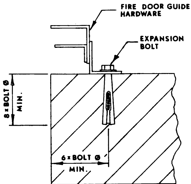
Figure B-10 Unusually thick walls.
