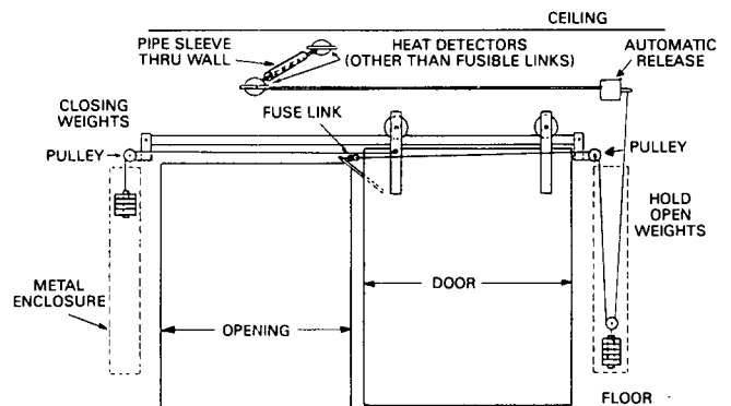
Figure B-36 Closing devices for single sliding door (level track).
