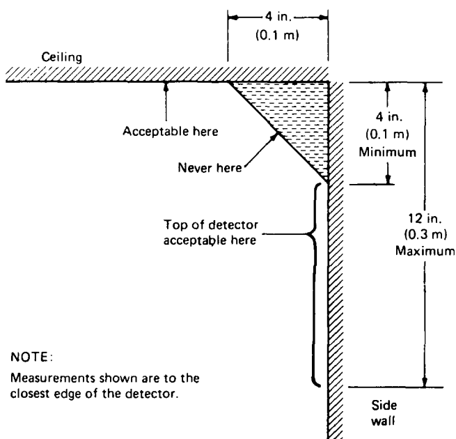
Figure B-59 Example of proper mounting for detectors.
