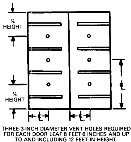
Figure B-33 Location of vent holes for swinging doors.
