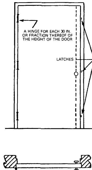
Figure B-22 Builders hardware (single swinging door with concealed three point latch — flush mounted).
