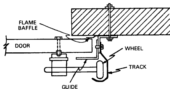
Figure B-47 Vertically sliding steel sectional overhead door.
