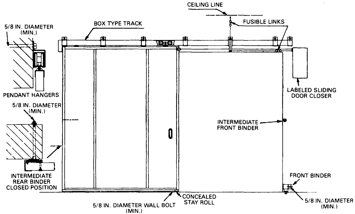
Figure B-41 Horizontally sliding composite door.
