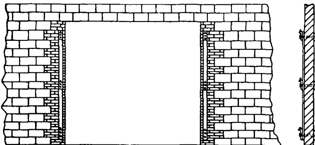
Figure B-16 Hollow concrete masonry wall prepared for doors swinging in pairs — lap mounted, standard method.
