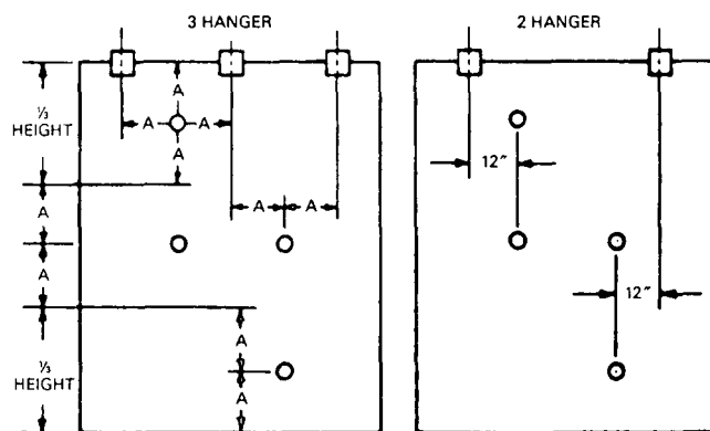
Figure B-40 Location of vent holes for horizontally sliding door.
