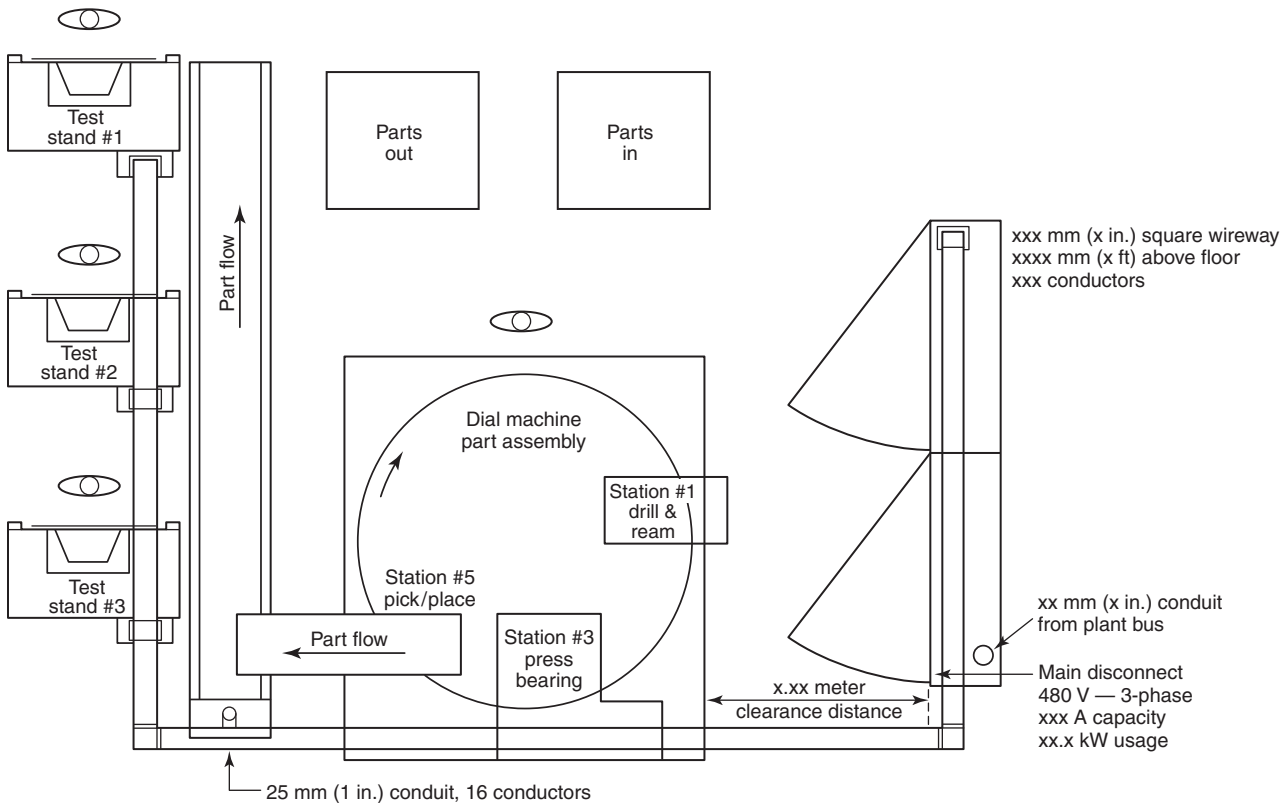
FIGURE D.1(b) System Layout and Installation Diagram.
