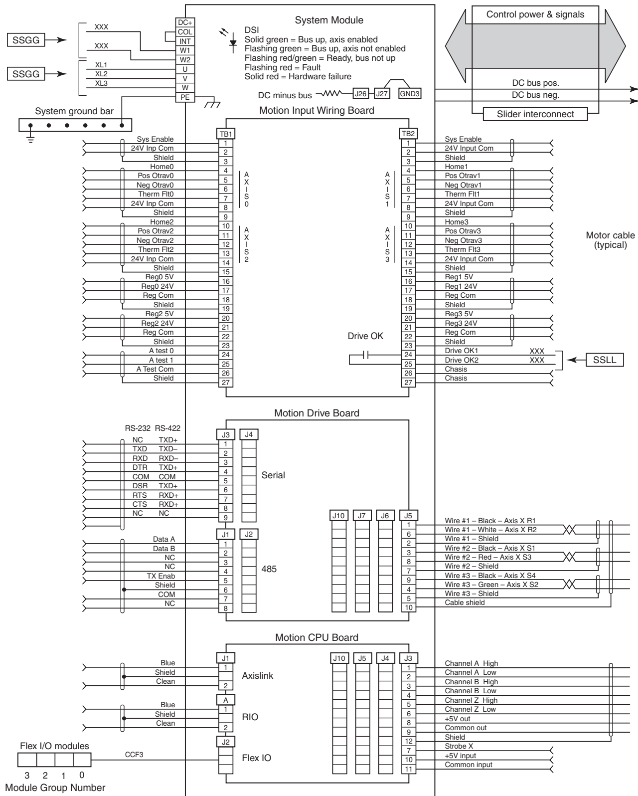
FIGURE D.1(I) Sample Servo Diagram.
