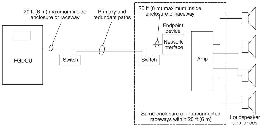
FIGURE A.5.4.3.6(1)(c) Class N Pathway to Endpoint with Multiple Devices. [72:Figure A.12.3.6(1)(c)]
