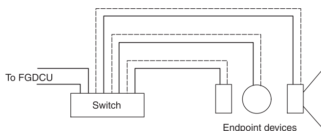
FIGURE A.5.4.3.6(1)(d) Class N Pathway Block Diagram with Multiple Control Units. [72:Figure A.12.3.6(1)(d)]
