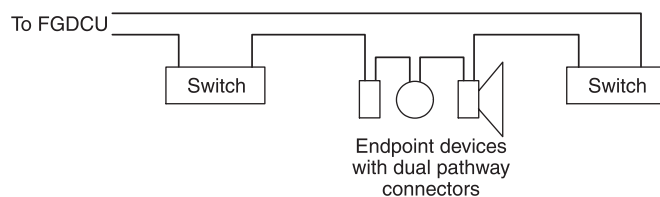
FIGURE A.5.4.3.6(5) Class N Pathway Block Diagram with Daisy-Chained Devices with Dual Pathway Connection. [72:Figure A.12.3.6(5)]
