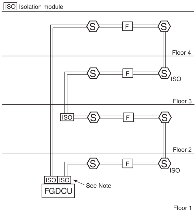
FIGURE A.5.6.1(a) Class B Isolation Method.
