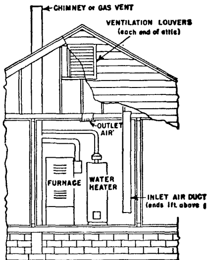
Fig. 3. Equipment Located in Confined Spaces; All Air from Outdoors Through Ventilated Attic. See 5.3.3-b.
