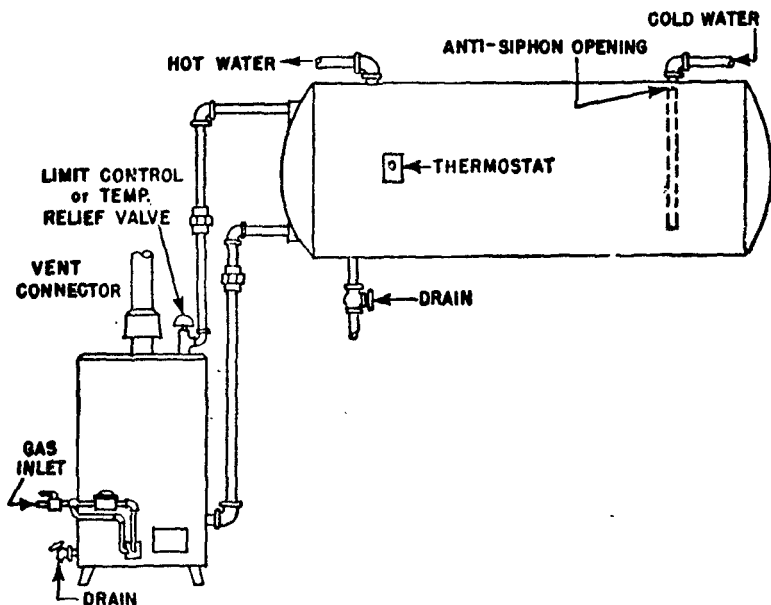
Fig. 9. Suggested Location for Anti-Siphon Opening in Cold Water Inlet.
