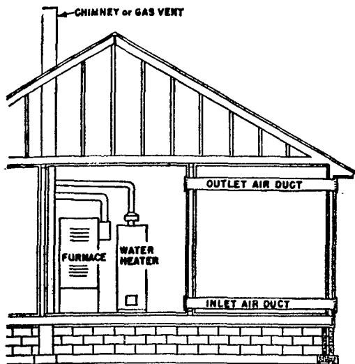
Fig. 3. Equipment Located in Confined Spaces; All Air from Outdoors Through Ventilated Attic. See 5.3.3-b.
