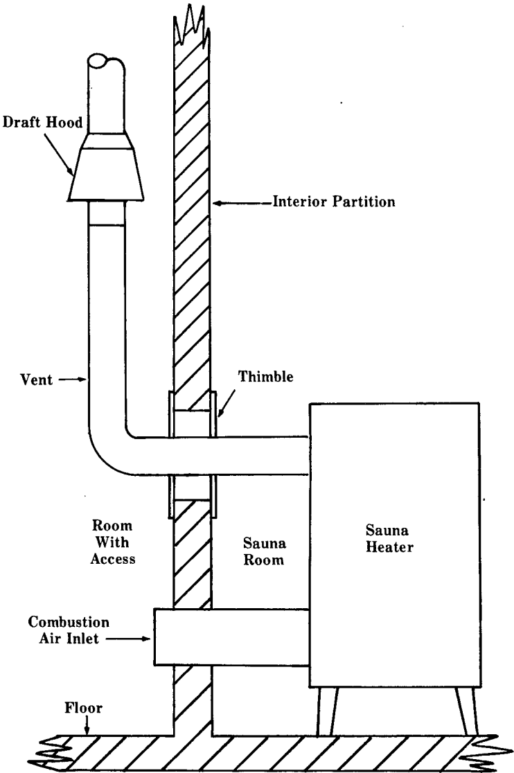
Fig. 7. Typical Sauna Heater Installation.
