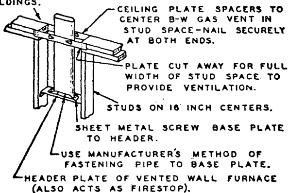
Fig. 8. Installation of Type B-W Gas Vents for Vented Wall Furnaces.
