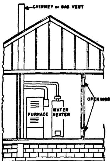
Fig. 1. Equipment Located in Confined Spaces; All Air from Inside the Building. See 5.3.3-a.
