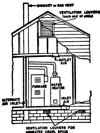
Fig. 2. Equipment Located in Confined Spaces; All Air from Outdoors — Inlet Air from Ventilated Crawl Space and Outlet Air to Ventilated Attic. See 5.3.3-b.
