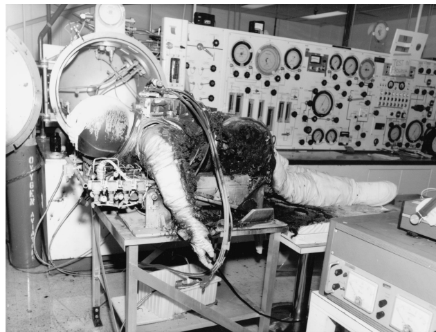
FIGURE D.2.6.7 Space Suit Destroyed in a Fire. No One Was in the Suit at the Time of the Fire. (Courtesy of NASA/Johnson Space Center.)
