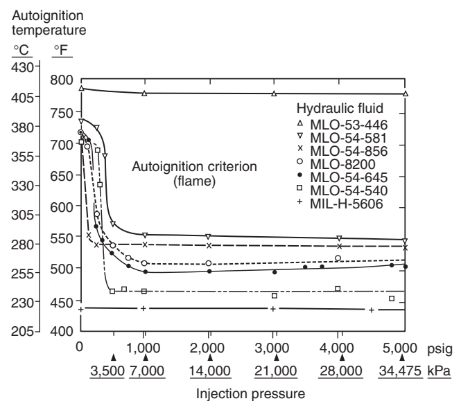
FIGURE F.2.2.1 Minimum Autoignition Temperatures of Seven Hydraulic Fluids in Air at Atmospheric Pressure and at Various Injection Pressures (200 cm 3 Pyrex ® Vessel). (13)
