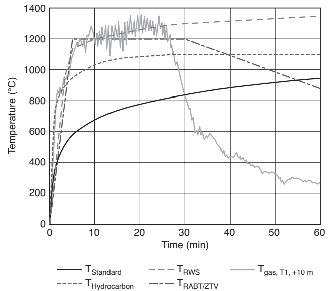
FIGURE A.7.3.2(c) Various Time-Temperature Curves and Fire Test Curve.
