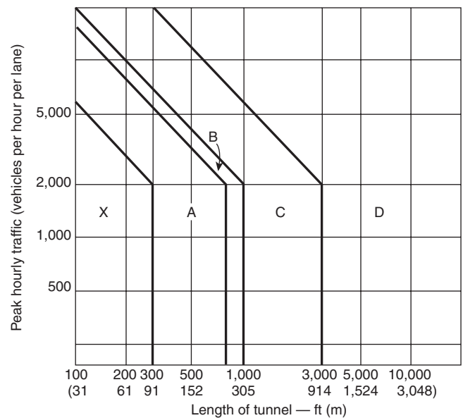
FIGURE A.7.2 Urban and Rural Tunnel Categories.
