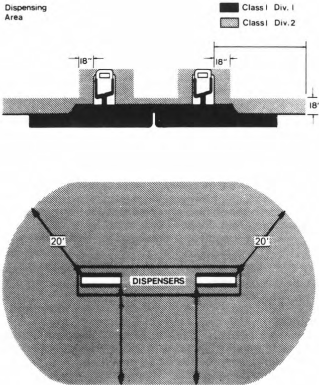
Figure 7-1 Classified areas adjacent to dispensers as detailed in Table 7.
