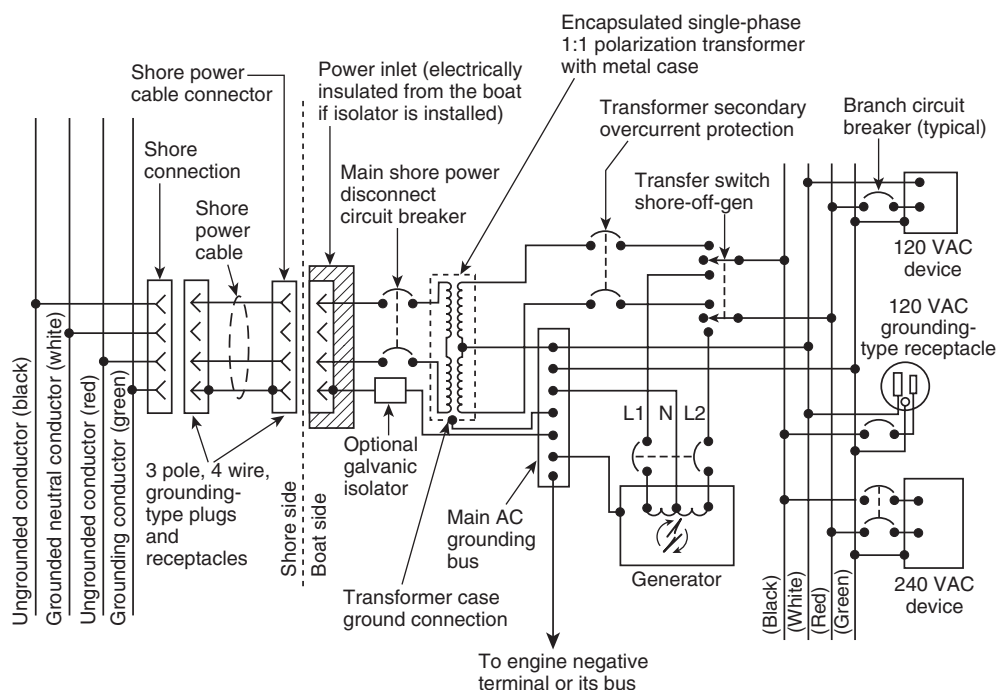
FIGURE 10.7.3(m) Polarization Transformer System — Single-Phase 240-Volt Input and 120/240-Volt Output — Generator with Main ac Grounding Bus.
