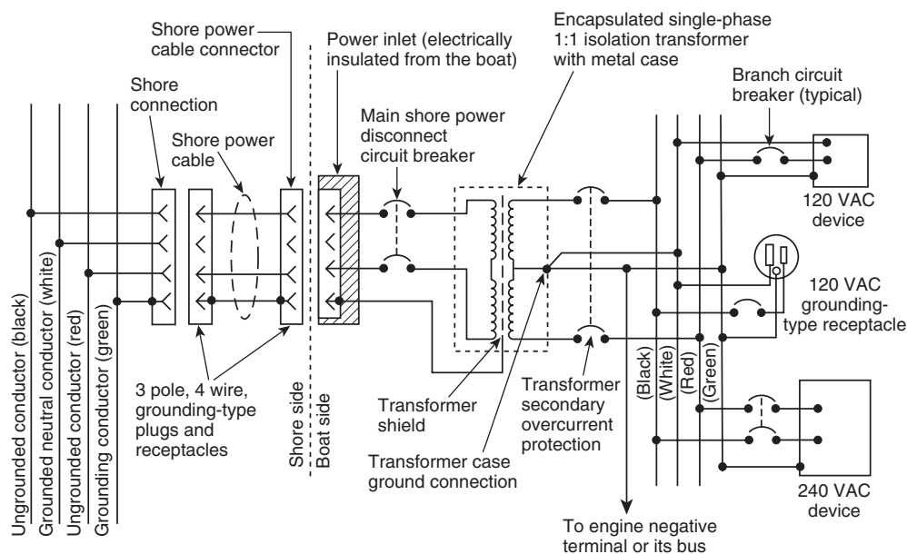
FIGURE 10.7.3(k) Isolation Transformer System — Single-Phase 240-Volt Input and 120/240-Volt Output with Boat-Grounded Secondary, Shore-Grounded Transformer Shield, and Boat-Grounded Transformer Metal Case.
