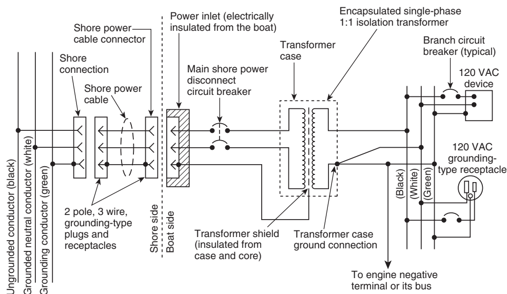
FIGURE 10.7.3(j) Single-Phase 120-Volt Isolation Transformer System with Boat-Grounded Secondary, Shore-Grounded Transformer Shield, and Boat-Grounded Transformer Metal Case.
