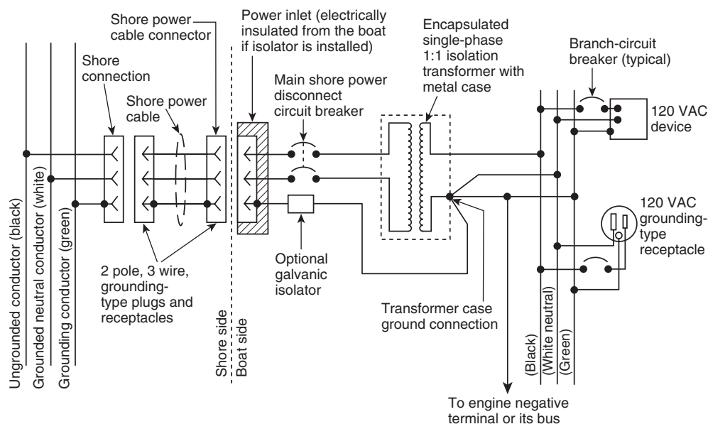
FIGURE 10.7.3(f) Single-Phase 120-Volt Polarization Transformer System with Shore Grounding Wire Protection of Transformer Primary.
