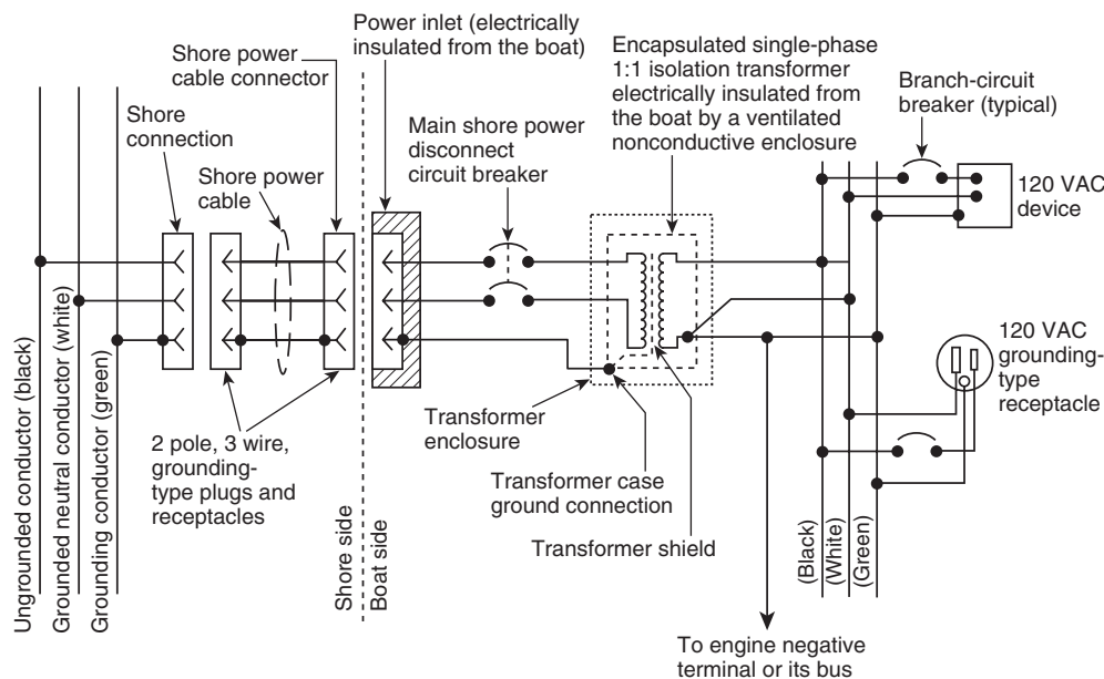
FIGURE 10.7.3(d) Single-Phase 120-Volt Isolation Transformer System with Grounded Secondary.
