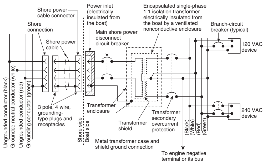
FIGURE 10.7.3(e) Isolation Transformer System with Single-Phase 240-Volt Input and 120/240-Volt Single-Phase Output.
