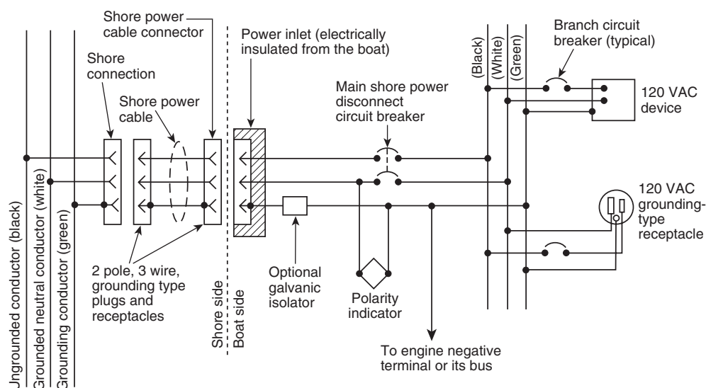
FIGURE 10.7.3(l) Single-Phase 120-Volt System with Polarity Indicating Device, Shore-Grounded Neutral Conductor, and Shore-Grounded Grounding Conductor.
