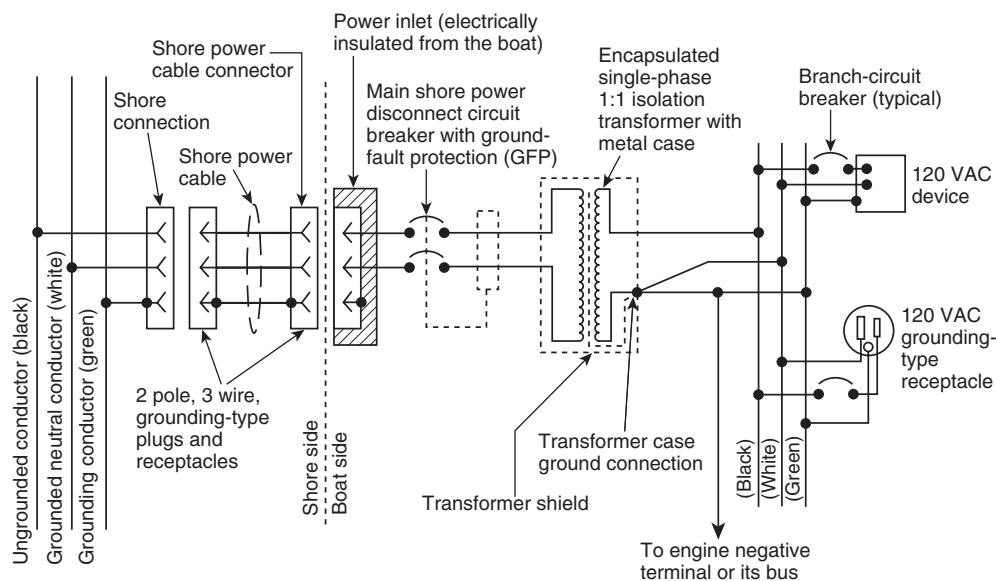
FIGURE 10.7.3(g) Single-Phase 120-Volt Isolation Transformer System with Ground-Fault Circuit-Interrupter (GFCI) Protection of Transformer Primary.
