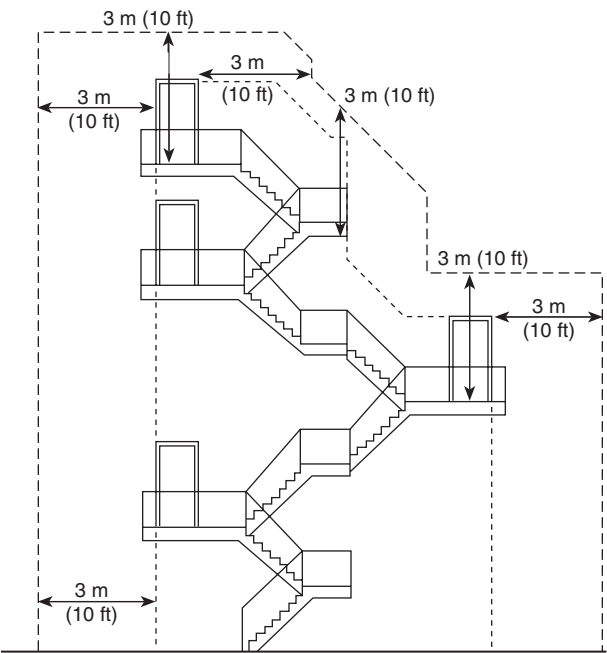
FIGURE A.7.2.2.6.2 Protection of Outside Stairs.
