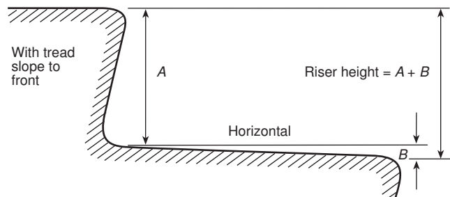
FIGURE A.7.2.2.2.3(a) Riser Measurement with Tread Slope to Front.
