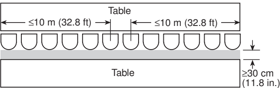
FIGURE A.7.2.11(b) Aisle Accessway Width ≥30 cm (11.8 in.).
