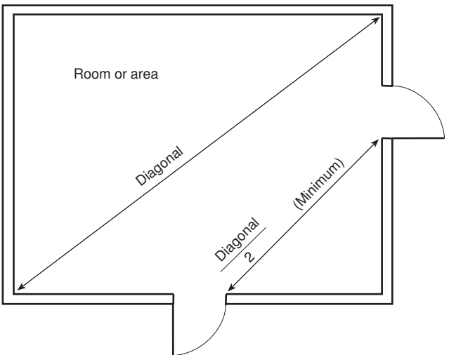
FIGURE A.7.5.1.5(a) Remoteness and Half-Diagonal Rule.
