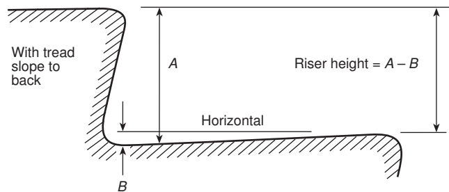
FIGURE A.7.2.2.2.3(b) Riser Measurement with Tread Slope to Back.
