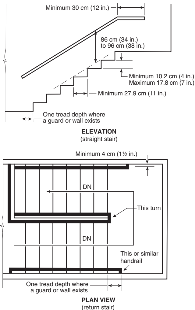
FIGURE A.7.2.2.4.5 Handrail Details.
