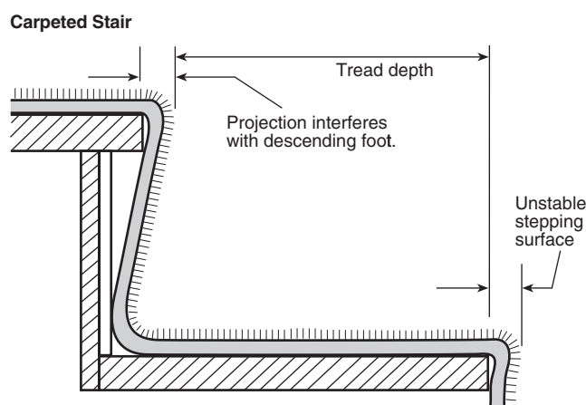
FIGURE A.7.2.2.3(e) Tread Measurement with Unstable Stepping Surface at Leading Edge.
