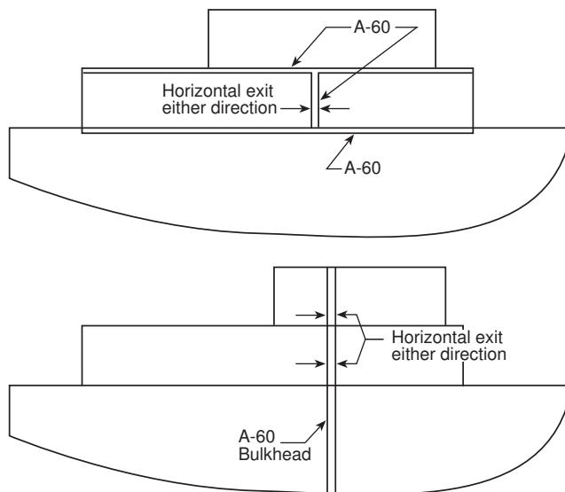
FIGURE A.3.3.23.1 Horizontal Exit.
