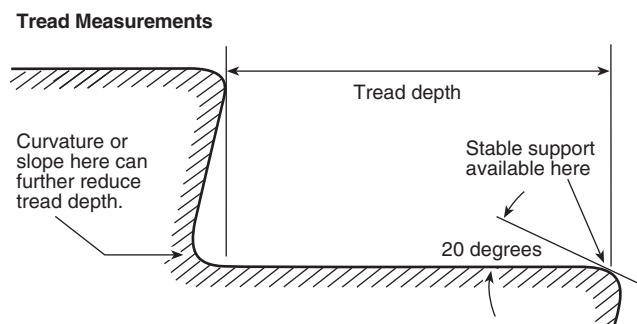
FIGURE A.7.2.2.3(d) Tread Measurement with Stable Support at Leading Edge.
