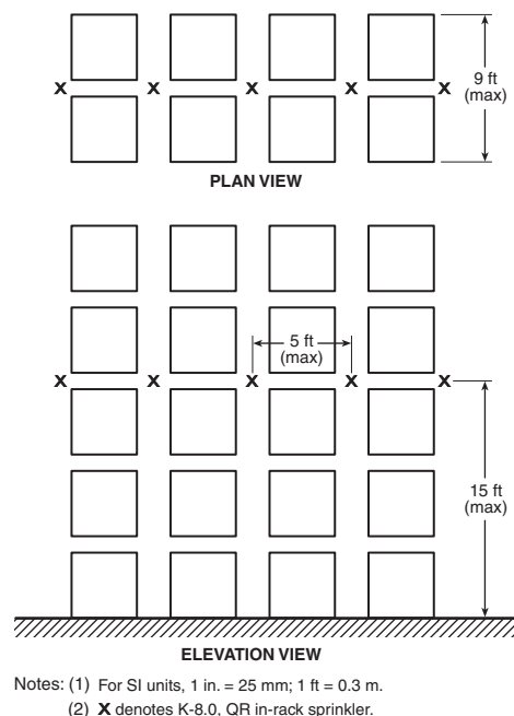
FIGURE 16.6.4(e) Double-Row Rack Sprinkler Layout H — Option #2.
