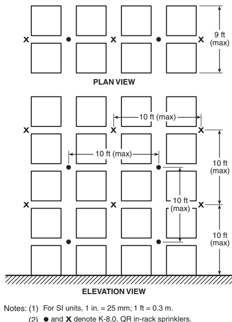
FIGURE 16.6.4(b) Double-Row Rack Sprinkler Layout I — Option #1.
