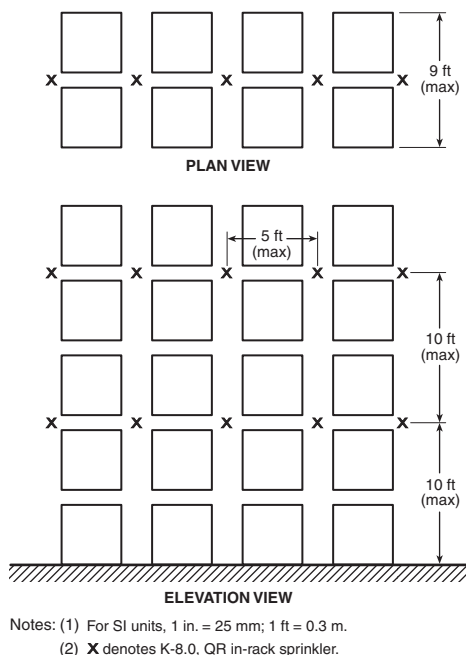
FIGURE 16.6.4(c) Double-Row Rack Sprinkler Layout I — Option #2.
