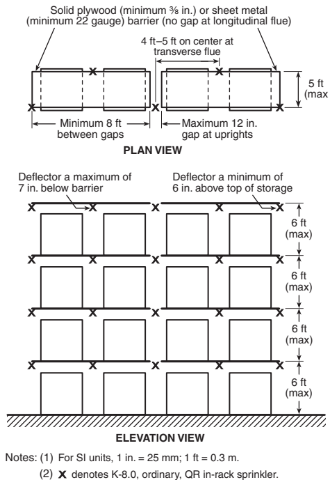
FIGURE 16.6.2.1(b) Double-Row Rack Sprinkler Layout for Design Scheme “B” — Sprinklers on Face of Rack.
