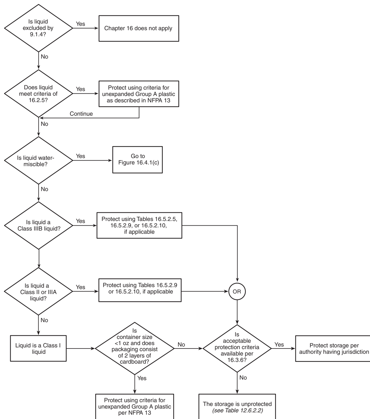
FIGURE 16.4.1(b) Fire Protection Criteria Decision Tree for Nonmiscible Flammable and Combustible Liquids in Nonmetallic Containers.
