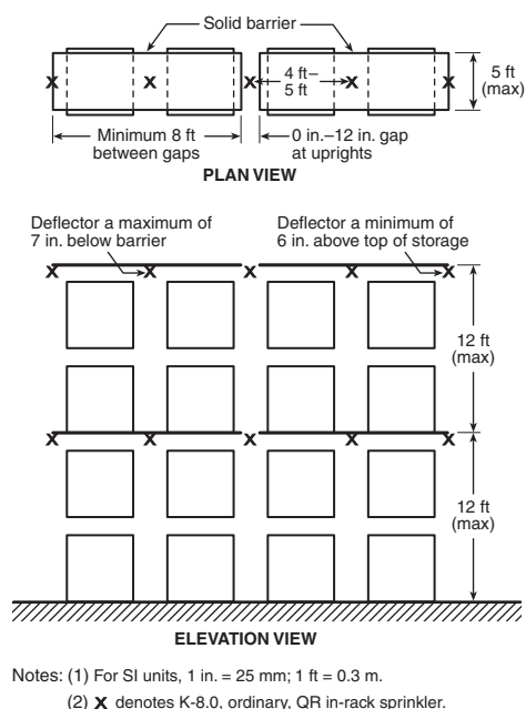
FIGURE 16.6.1.1(a) Single-Row Rack Sprinkler Layout for Design Scheme “A.”
