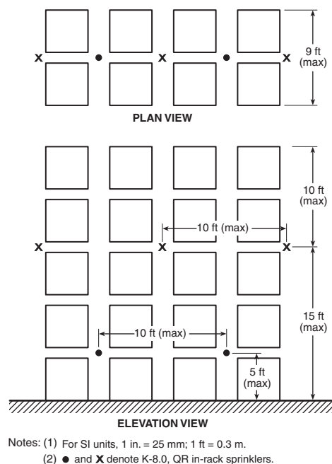
FIGURE 16.6.4(d) Double-Row Rack Sprinkler Layout H — Option #1.
