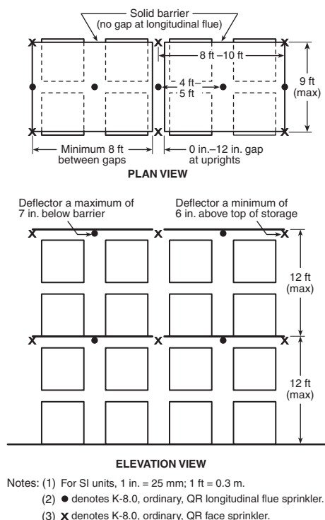
FIGURE 16.6.1.1(b) Double-Row Rack Sprinkler Layout for Design Scheme “A.”
