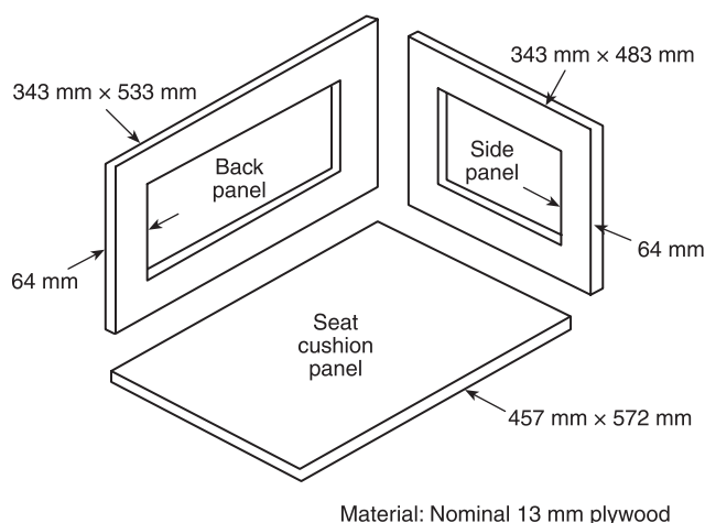
FIGURE 4.1(c) Panels for Upholstered Furniture Mock-Up Test.
