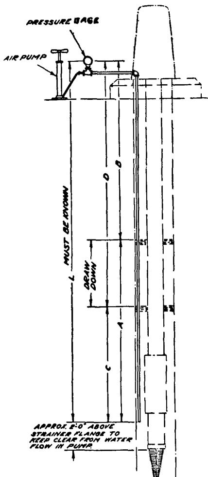
Fig. 236. Air Line Method of Determining Depth of Water Level.
