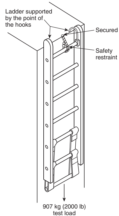
FIGURE 5.3.1 Design Verification Roof Hook Test.
