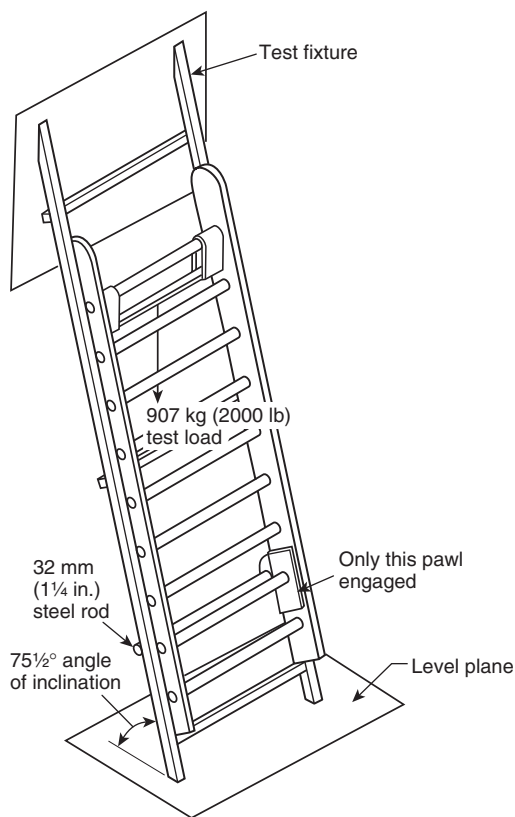
FIGURE 5.4.2.2 Design Verification Single Pawl Load Test.
