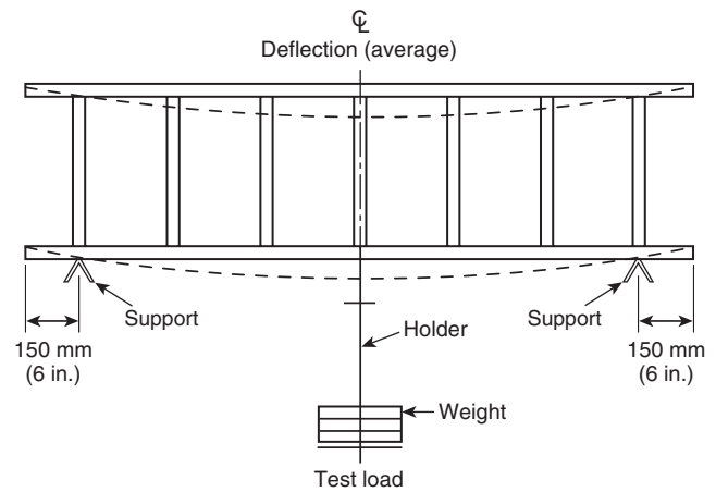
FIGURE 5.2.6.2 Position of Ladder for Design Verification Side Sway Test.
