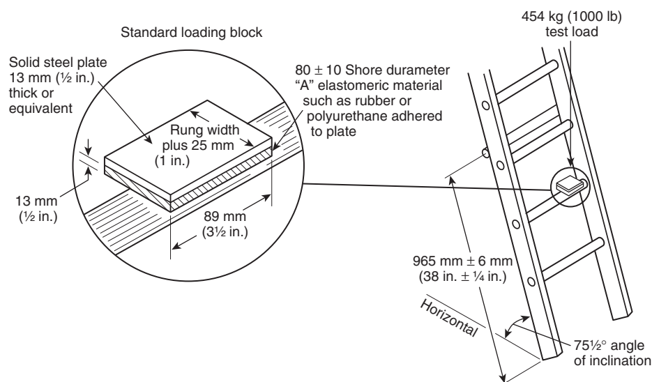
FIGURE 5.2.4.1.1 Design Verification Rung-to-Beam Shear Strength Test.
