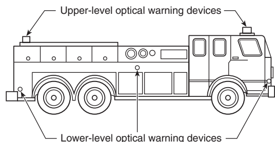
FIGURE A.13.8.1 Upper- and Lower-Level Optical Warning Devices. [1901:Figure A.13.8.1]
