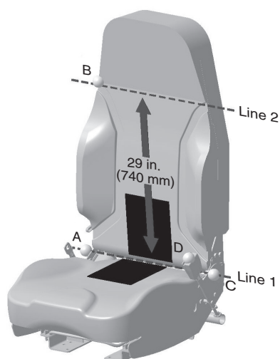
FIGURE 14.1.3.2 Dimension Lines for Measuring Seat Belt Effective Length. [1901: Figure 14.1.3.2]
