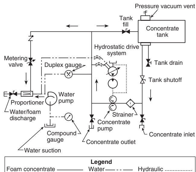
FIGURE A.20.2.5(c) Demand Balanced Pressure Foam Proportioning System. [1901:Figure A.20.2.5(c)]
