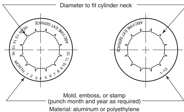
FIGURE A.11.3.1.2.5 Design of a Verification-of-Service Collar. [10:Figure A.7.11]
