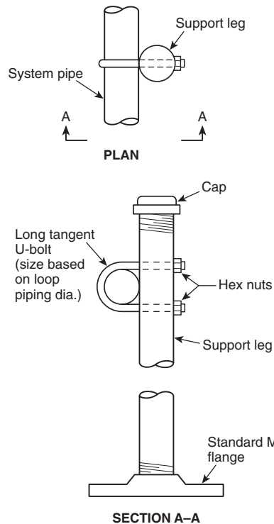
FIGURE A.6.3.2.2.5(c) Acceptable Attachment for Pipe to Support Legs — Example 2.
