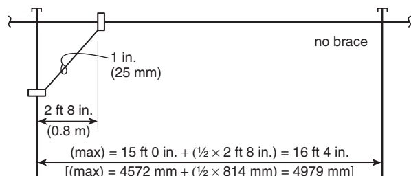
FIGURE A.6.3.2.2.2 Sway/Support Brace.
