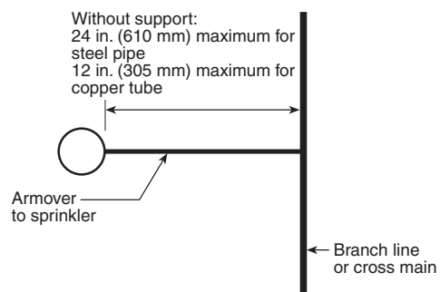
FIGURE A.9.2.3.5 Maximum Length for Unsupported Armover.
