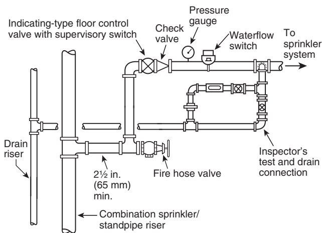
FIGURE A.8.17.5.2.2(b) Acceptable Piping Arrangement for Combined Sprinkler/Standpipe System. [14:Figure A.7.10.1.3.1(b)]
