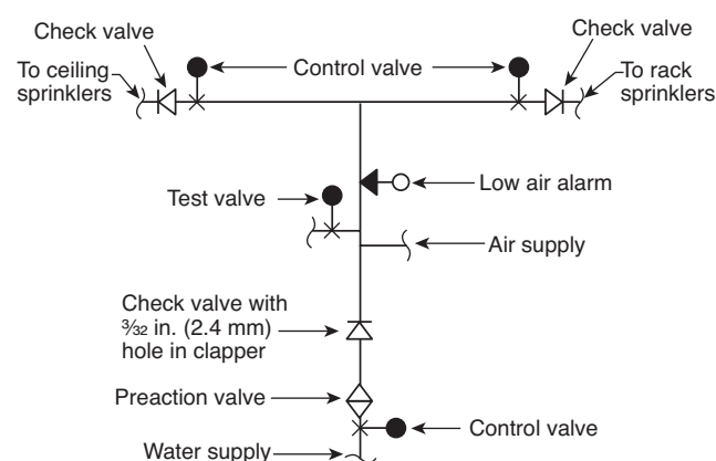
FIGURE 7.9.2.8.4 Valve Arrangement.
