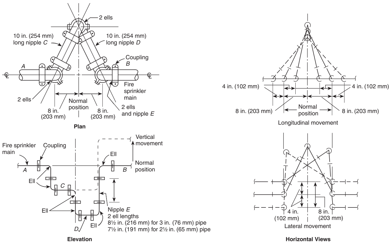
FIGURE A.9.3.3(a) Seismic Separation Assembly. Shown are an 8 in. (203 mm) Separation Crossed by Pipes up to 4 in. (102 mm) in Nominal Diameter. For other separation distances and pipe sizes, lengths and distances should be modified proportionally.
