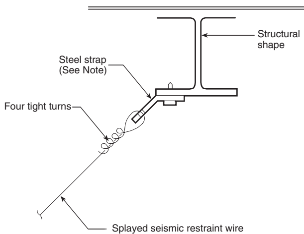
Detail A — At steel beams
