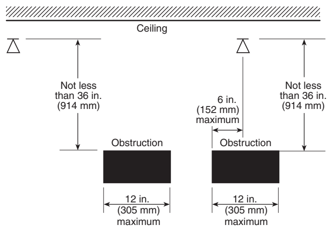
FIGURE 8.11.5.3.5 Obstruction More Than 36 in. (914 mm) Below the Sprinkler (Large Drop Sprinkler).
