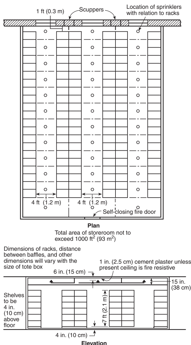
FIGURE 21.8.2.5(a) Tote Box Storeroom Showing General Arrangement of Racks and Sprinklers. [42:Figure 6.7]
