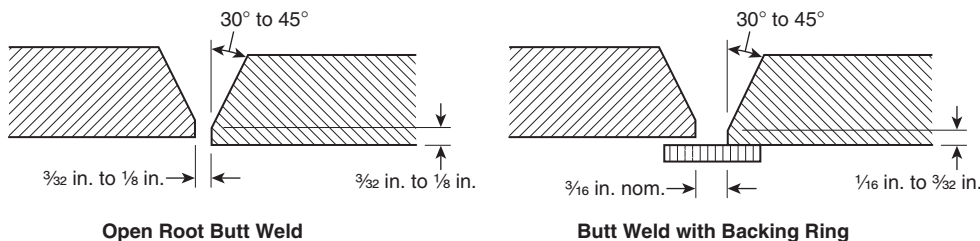
FIGURE A.6.5.2.2 Weld Diagram.
