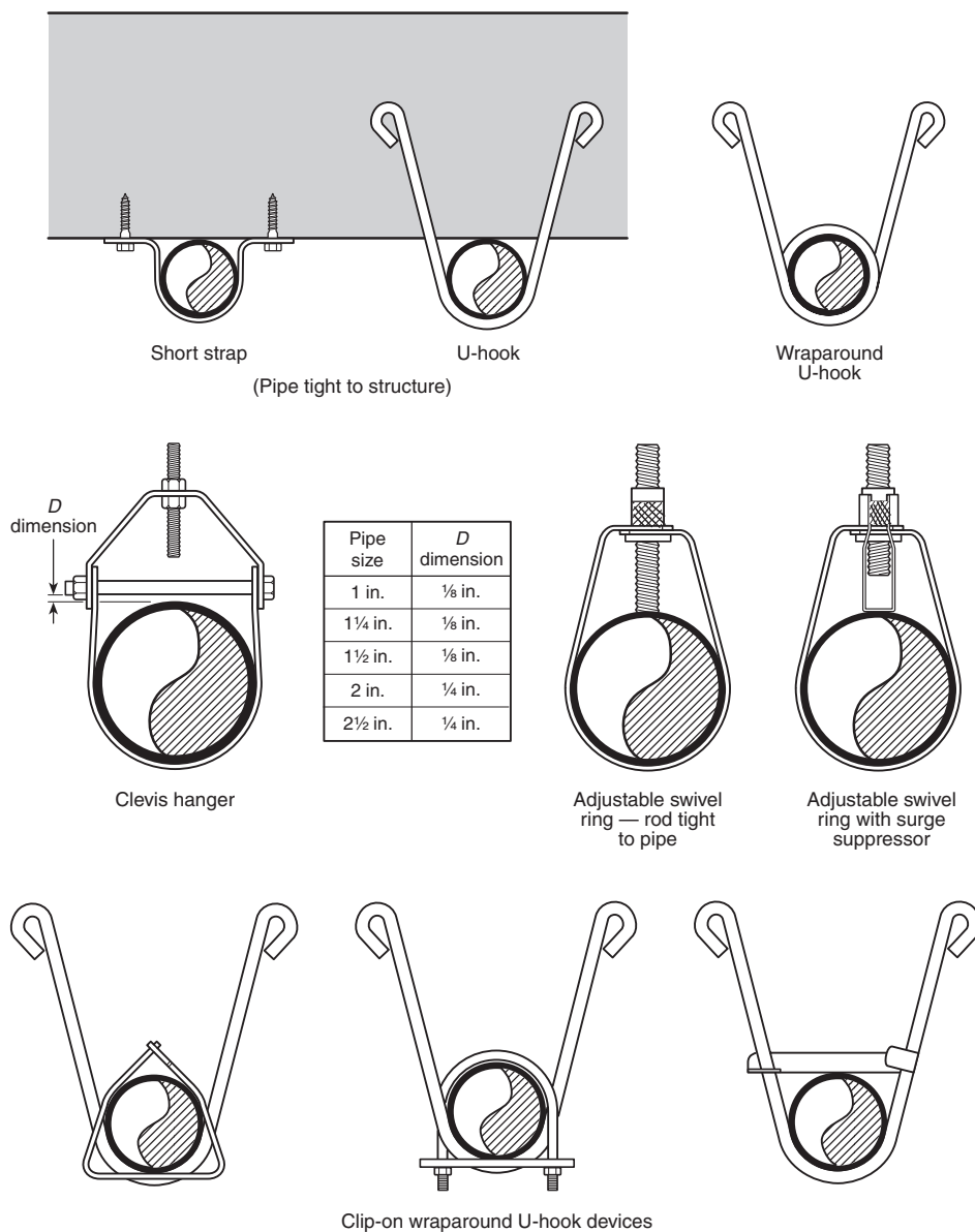
FIGURE A.9.2.3.4.4(b) Examples of Acceptable Hangers for End-of-Line (or Armover) Pendant Sprinklers.
