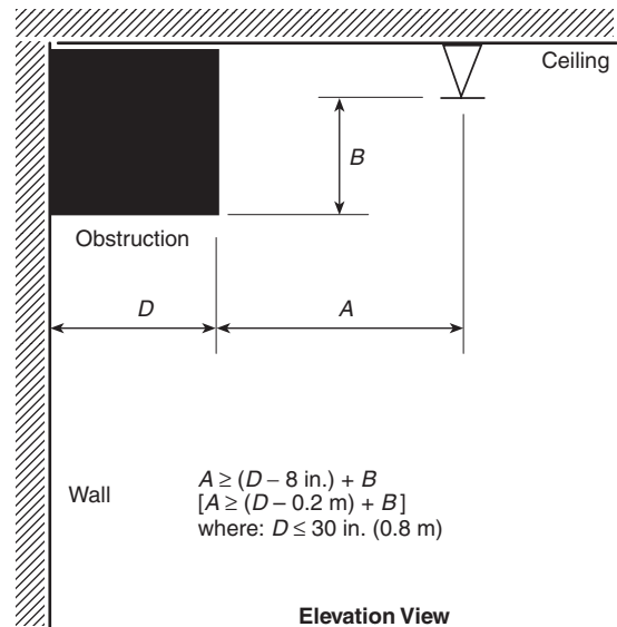
FIGURE 8.10.6.1.2(b) Obstructions Against Walls (Residential Upright and Pendent Spray Sprinklers).
