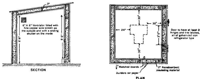
Fig. 5258-5. Dry-Pipe Valve Enclosure — Combustible Construction.
