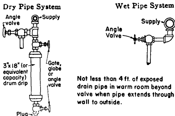
Fig. 3230. Auxiliary Drains.
