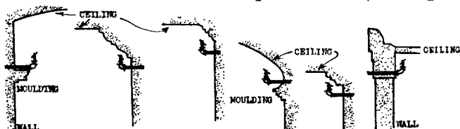
Fig. 4430. Suggested Arrangements for Sidewall Sprinklers—placed to receive early heat waves and provide effective distribution.
