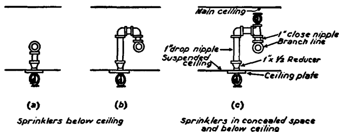
Fig. 3066. Pendent Sprinklers at Suspended Ceiling.
