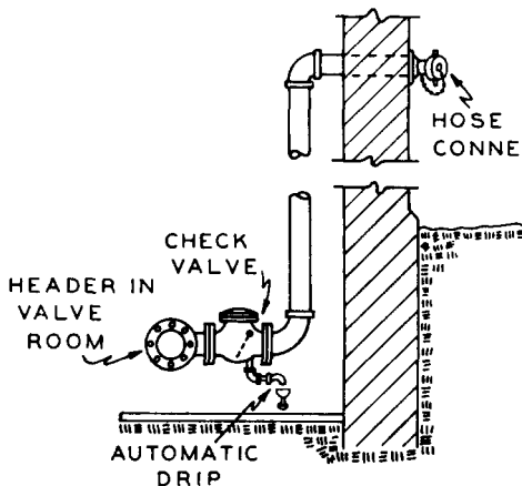
Fig. 2600. Fire Department Connection.
