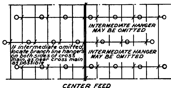
Fig. 3574. Hangers on Cross Main — Center Feed System.
