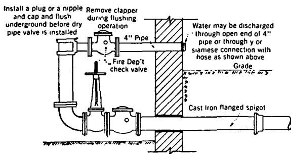
Fig. 1621. Methods of Flushing Water Supply Connections.
