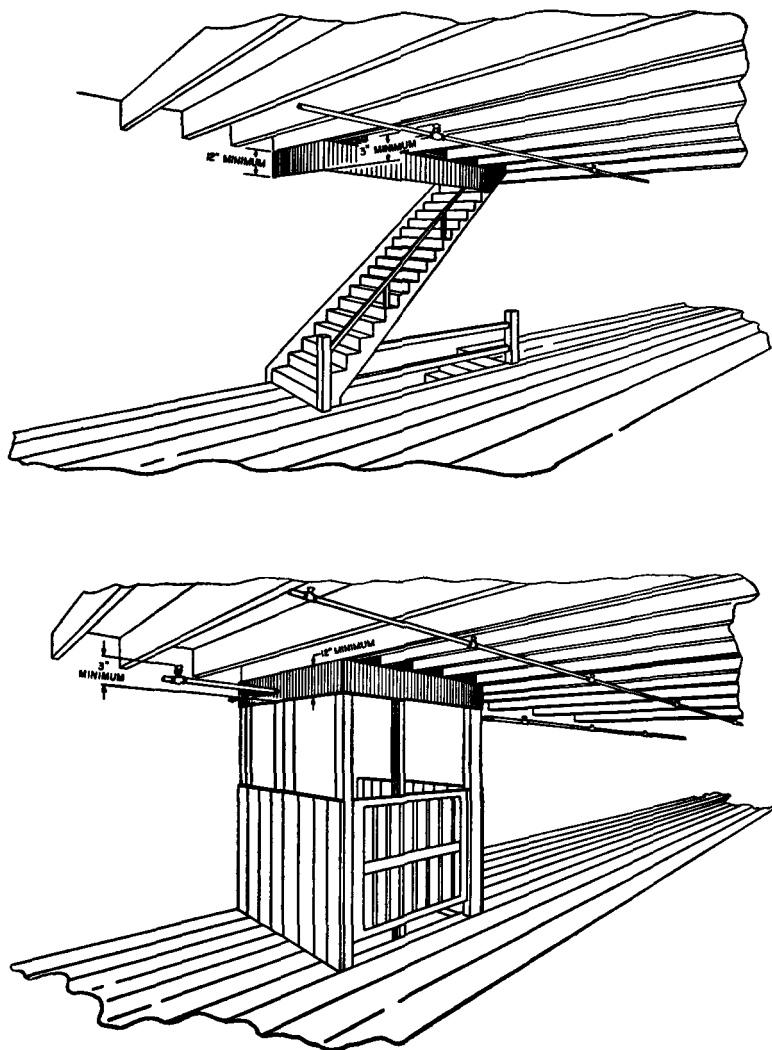
Fig. 1132. Draft Curtains around Open Stair and Elevator Shafts. Preferably of noncombustible material such as flat sheet or corrugated metal.
