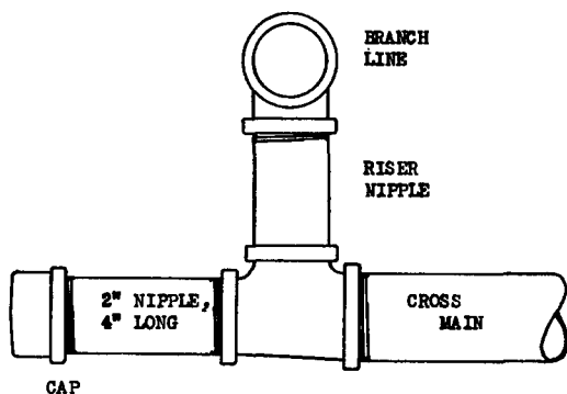
Fig. 3063. Flushing Connection.
