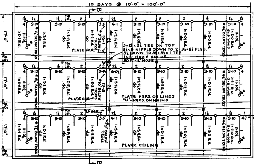
Fig. 1440-2. Typical Working Plans (cont.)
