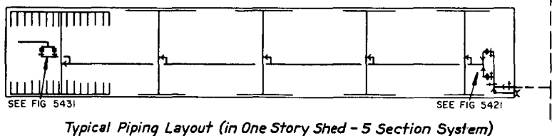
Fig. 5411. Typical Piping Layout for Combined Dry-Pipe and Pre-Action Sprinkler System.
