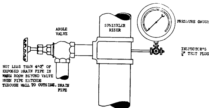
Fig. 3220. Drain Connection for Sprinkler Riser.
