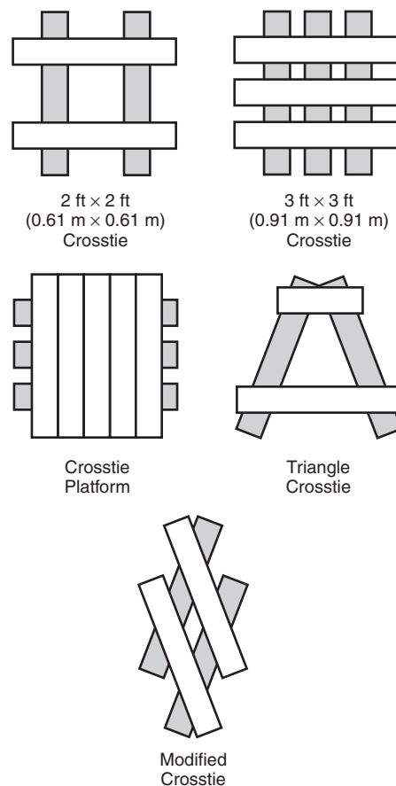
FIGURE A.9.1.13 Five Basic Configurations of Cribbing.
