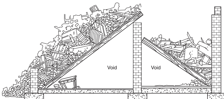
FIGURE B.1(e) A-Frame Floor Collapse. (Courtesy of U.S. Department of Civil Defense)
