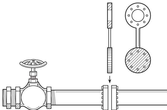
FIGURE A.7.2.2 Blanking or Blinding.
