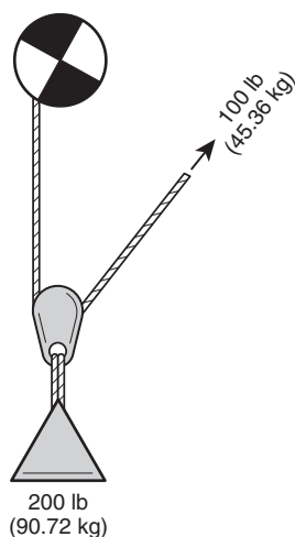
FIGURE A.3.3.121.2 A Simple Rope 2:1 Mechanical Advantage System.
