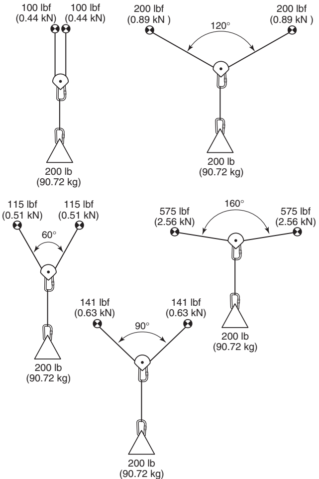
FIGURE A.6.1.3(A) The Effect of Angle Forces on Anchors and Lines: Critical Angles.
