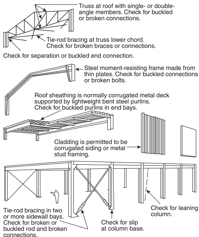
FIGURE D.1(a) Light Metal Building.
