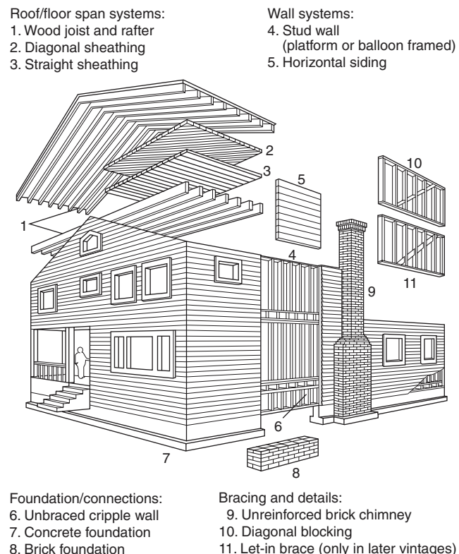
FIGURE D.1(c) Wood Stud Frame Construction.
