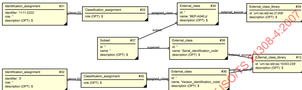
Figure 8 — Classification of individual root instantiation diagram
