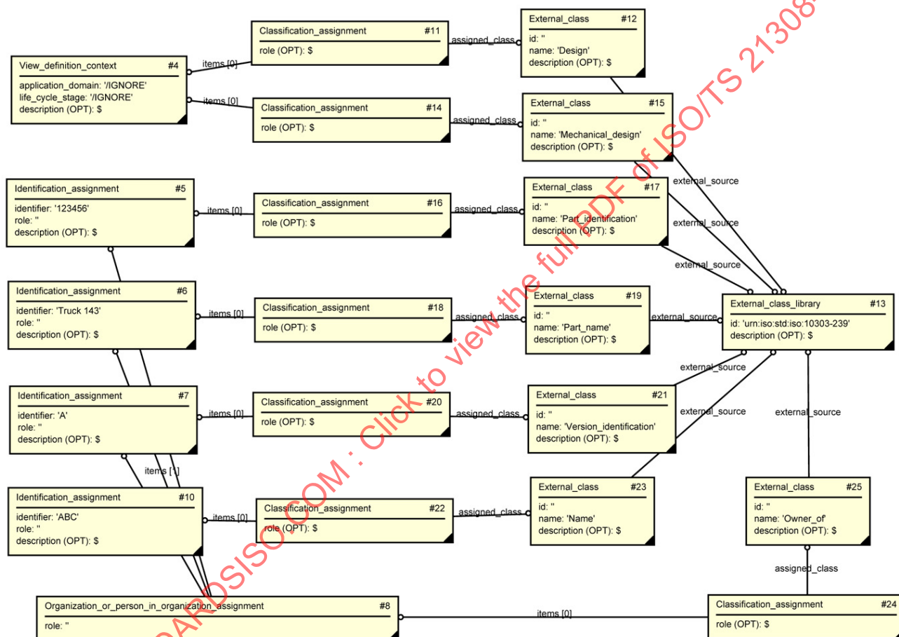
Figure 6 — Classification of part instantiation diagram
