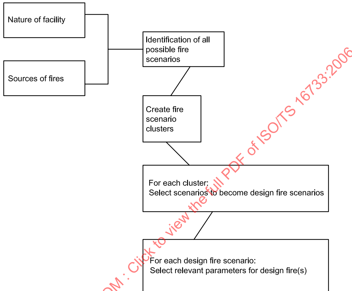
Figure 1 — Selection of design fire scenarios and design fires
