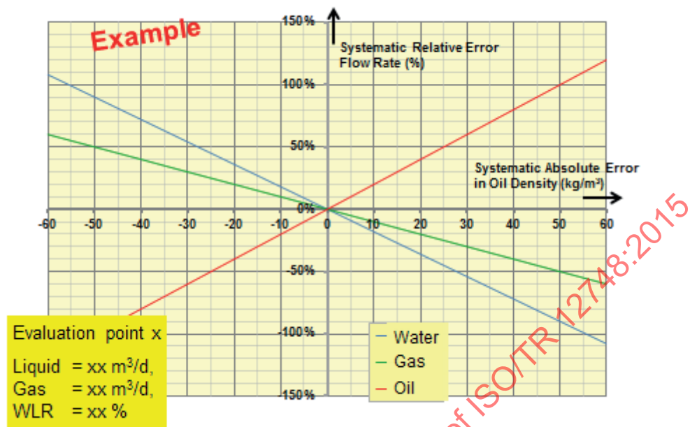
Figure 37 — Hypothetical example of fluid property input error vs. WGFM output bias
