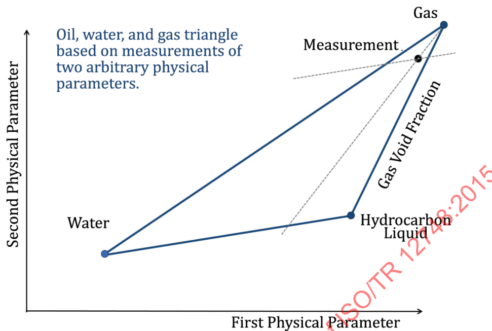
Figure 20 — A water, light liquid hydrocarbon and gas triangle plotted for measurements of two arbitrary physical parameters
