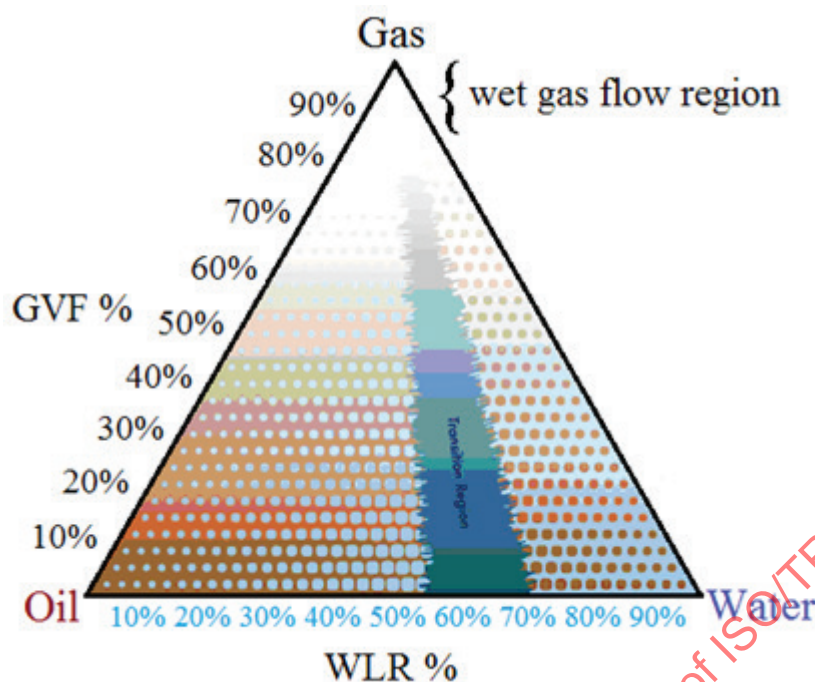
Figure 19 — An example of a multiphase composition triangle
