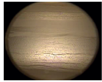
c) Transition between stratified and annular mist
