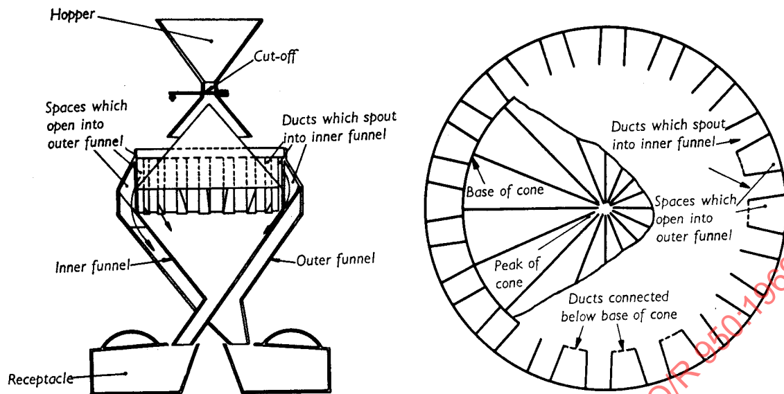
FIG. 8 — Conical divider (Boerner type)
