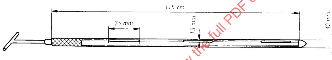
FIG. 4 — Cylindrical sampler (divided bulk probe)
