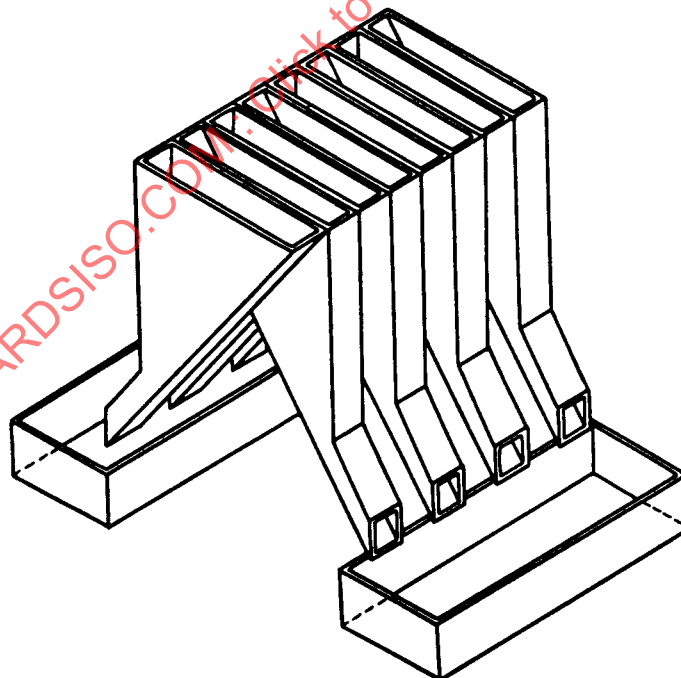
FIG. 9 — Multiple-slot divider
