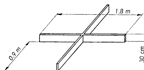
FIG. 7 — Quartering irons
