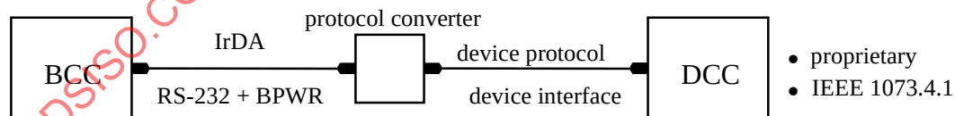
Figure A.3—Physical configuration with a protocol converter
