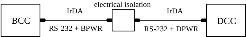
Figure A.4—Physical configuration with electrical isolation
