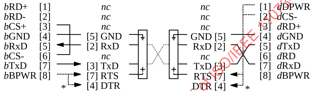
BCC to DTE DB-9M [ fiber optic ] DTE DB-9M to DCC line-extender
