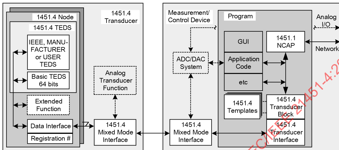
Figure 3—IEEE 1451.4 TEDS data system block diagram
