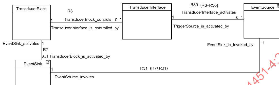
Figure 34—IEEE1451_Dot4EventSink associations
