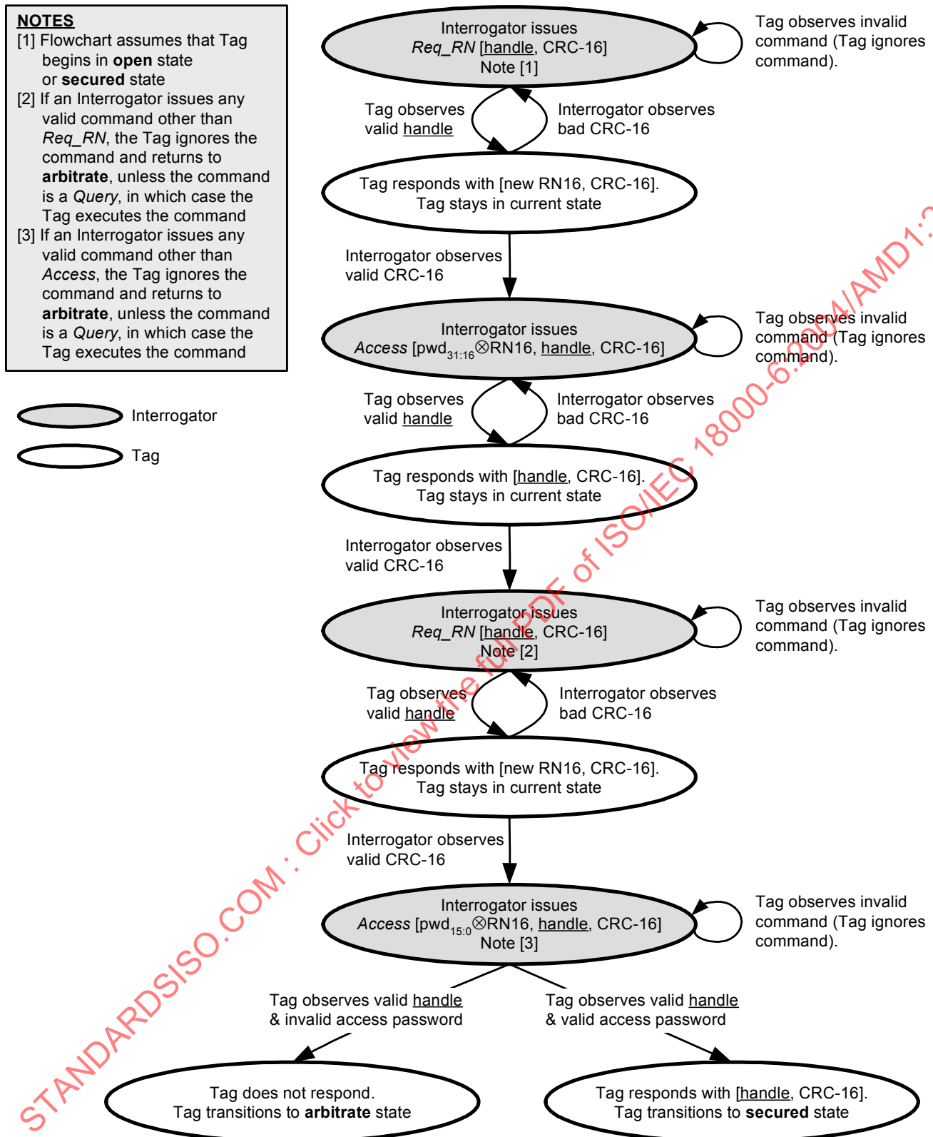
Figure Amd.1-28 — Access procedure
