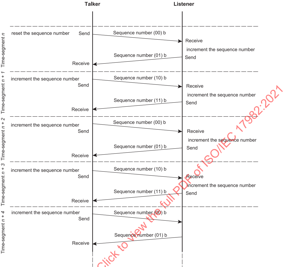
Figure 13 — Example flow of full duplex communication
